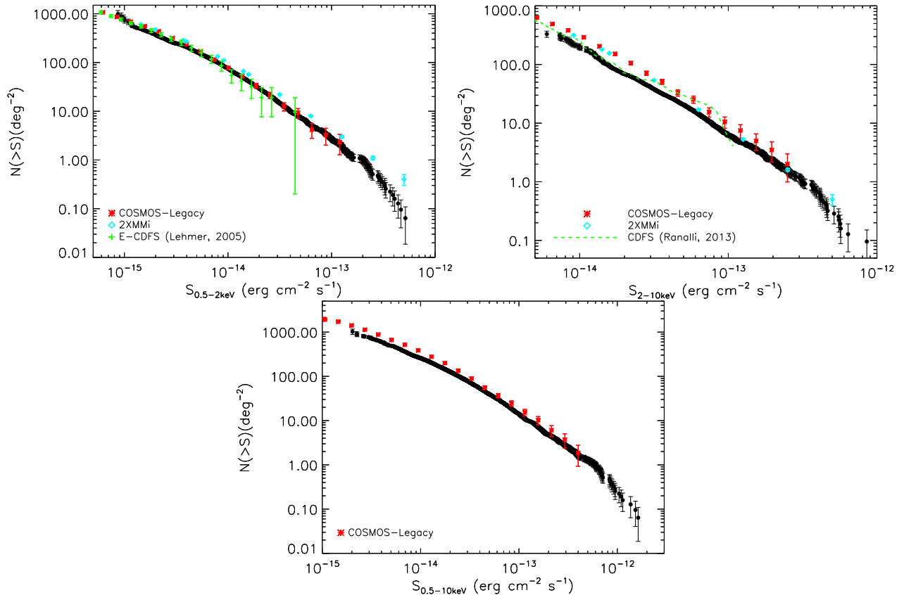
FIG. 3.— Cumulative Log N -Log S relationship for the Stripe 82X survey ( black circles ) in the soft ( top left ), hard ( top right ), and full ( bottom ) bands. For reference, we also plot the source number density for other surveys, spanning the gamut from deep, pencil-beam surveys (i.e., the 0.3 deg 2 ECDF-S and \sim 0.25 deg 2 CDFS; Lehmer et al. 2005; Ranalli et al. 2013, respectively), to a moderate-area, moderate depth survey (the 2.2 deg 2 Chandra COSMOS-Legacy; Civano et al., submitted , Marchesi et al., submitted ), and a wide-area survey (the 132 deg 2 2XMMi Serendipitous Survey; Mateos et al. 2008).
