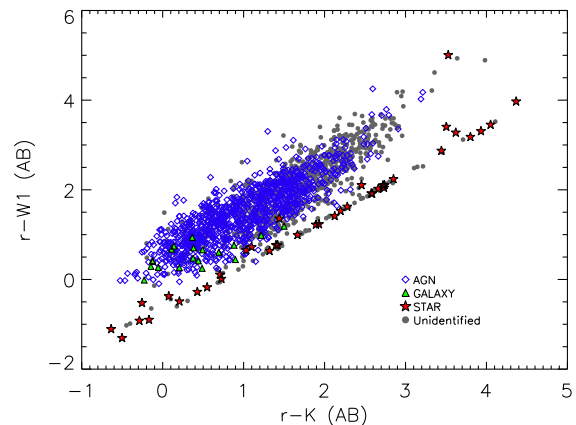
FIG. 12.— r-W1 (AB) color as a function of r-K (AB) color for the 1891 X-ray sources with SDSS, UKIDSS, and WISE counterparts that have K -band and W1 detections and UKIDSS ( WISE ) coordinates within 2'' (3'') of the SDSS position. Many of the stars can be identified by the distinct track they occupy in this color space (LaMassa et al. 2015).
