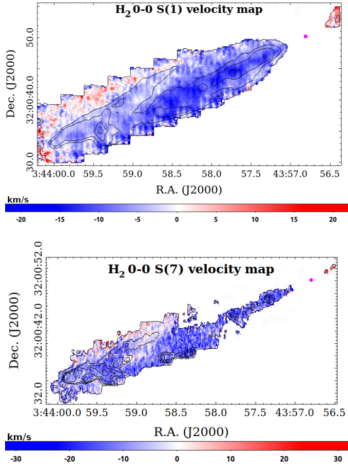
Fig. D.2. Top panel: H 2 velocity map of the 0-0 S(1) at 17 μm. Black contours show the integrated continuum-subtracted line intensity at 5, 10, 50, 100, and 200 \sigma (namely, 0.5, 1, 5, 10, and 20 mJy pixel -1 ). Bottom panel: H 2 velocity map of the 0-0 S(7) at 5 μm. Black contours show the integrated continuum-subtracted line intensity at 5, 50, 100, 200, and 500 \sigma (namely, 0.1, 1, 2, 4, and 10 mJy pixel -1 ). Only velocities within a 5 \sigma threshold are plotted in both panels. The magenta circle shows the position of the ALMA mm continuum source.
