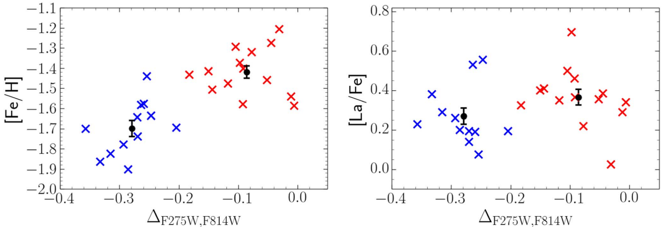
Figure 10. [Fe/H] and [La/Fe] abundances as a function of the \Delta_{F275W,F814W} axis of the ChM for M54. Blue and red crosses represent the stars associated with the red- and blue- RGB/ChM sequence, respectively, as in Figure 8. In each panel, we indicate the mean abundances with the associated error for each group.
