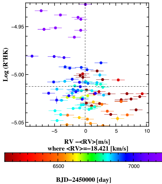
Fig. 6. Star activity index as a function of the radial velocity residuals after removing the three shorter-period planet contributions for HD 219134. No clear positive correlation is observed, contrary to what is expected in the case of magnetic cycles (Lovis et al. 2011a).
