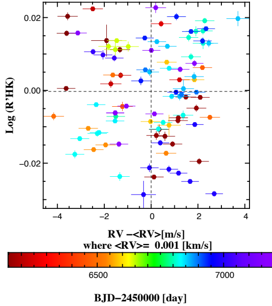
Fig. 8. Radial velocities after subtracting the contributions of the planets at 3.09, 6.76, and 1842 days, shown as a function of the \log R'_{\text{HK}} activity index detrended with a polynomial of degree 3. No correlation is observed, supporting the planetary interpretation for the 46.7-day signal.
