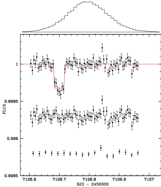
Fig. 11. Spitzer photometry divided by the best-fit baseline model and binned per 0.005\text{d} = 7.2 min, with the best-fit transit model overplotted in red. Below are shown the y -shifted residuals of the fit binned per 7.2 min and 30 min intervals. Their standard deviations are, respectively, 57 ppm and 25 ppm. Over the light curve is shown the prior probability distribution function derived for the transit timing of HD 219134 b from our analysis of the HARPS-N RVs.
