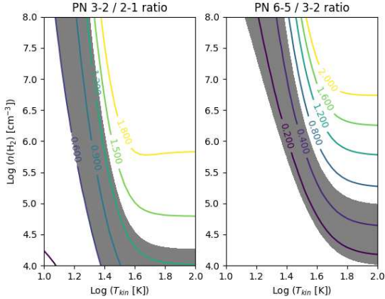
Figure 5. Predicted intensity ratios (coloured curves) of the PN 3–2/2–1 (left) and 6–5/3–2 (right) lines, calculated with RADEX for PN column densities of 10^{12} \text{cm}^{-2} . The gas temperatures range from 10 to 100 K and the densities from 10^4 to 10^8 \text{cm}^{-3} . The observed ranges are indicated by a grey area. As described in Sect. 3.2, this plot is used to derive n(\text{H}_2) from the line ratios and T_{\text{kin}} given in Table 4.
