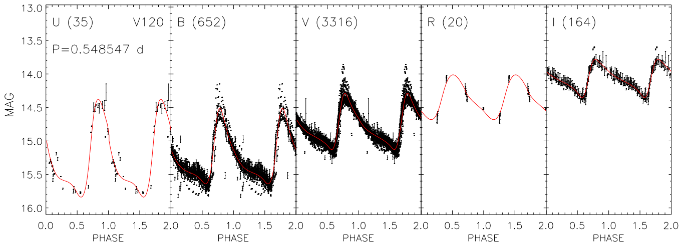
Figure 5. Same as Figure 3, but for the candidate Blazhko variable V120.
