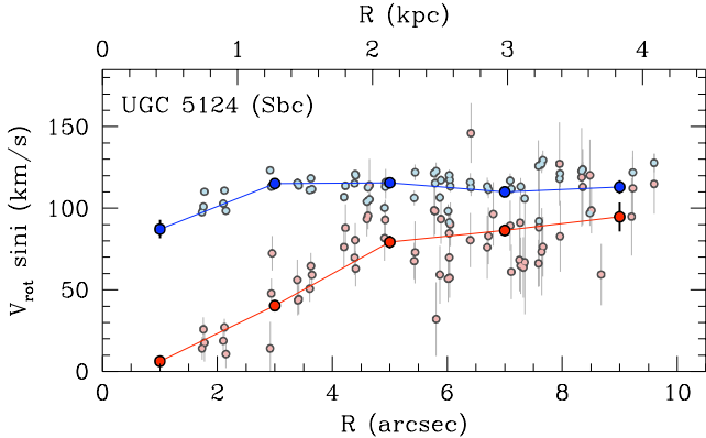
FIG. 16.— Detection of asymmetric drift in the MaNGA prototype observations of UGC 5124 (p9-61A), which has an inclination of i = 45.6 \pm 2.0^\circ and a distance of 87.8 Mpc. Small, light-blue and light-red points are measurements of ionized-gas and stellar velocities, respectively, as a function of disk-plane radius ( R ) from individual fibers that have been projected onto the major axis of rotation. Only those data within \pm 60^\circ (disk-plane azimuth) of the major axis have been plotted. Large blue and red points show the error-weighted mean, projected rotation speed ( V_{\text{rot}} \sin i ) in 2'' bins for the ionized-gas and stellar components, respectively. As expected, the stellar (red) component lags behind the ionized-gas (blue) component owing to the substantially larger velocity dispersion and collisionless nature of the stars.
