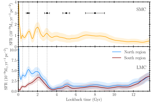
Figure 2. Comparison of the global SFHs for the SMC (this work) and the LMC (Ruiz-Lara et al. 2020b). Vertical dashed lines link the peaks at 0.45, 1.1, 2, and 3 Gyr ago in the SMC to those of the LMC. The horizontal bars show the width of the SFH enhancement. Uncertainties in the SFHs (shaded regions) were calculated as in Hidalgo et al. (2011) and Rusakov et al. (2021).
