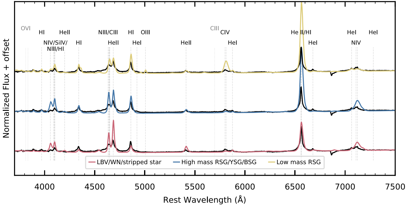
Figure 4. The day 1.36 spectrum (black) compared with three different surface abundance models from Boian & Groh (2019) with L = 1.5 \times 10^9 L_\odot , and \dot{M} = 3 \times 10^{-3} M_\odot \text{ yr}^{-1} . The solar abundance represents a low-mass RSG (yellow), CNO-processed abundance represents a high-mass star (RSG, BSG, or YSG; blue), and He-rich abundance represents an LBV, WN, or other stripped star (pink). Vertical dashed lines represent the ions that are identified in the observed spectra that are labeled at the top of the plot. Vertical dotted lines in light gray show ions that are not detected but are part of the progenitor diagnostics detailed in Boian & Groh (2019). We convolve the model spectra with a Gaussian kernel to mimic the resolution of the observed spectra. While some individual features in each model are matched by the observed spectrum, there are differences between the model and observed spectrum that indicate that the conditions of the model are not the same as the observations.
