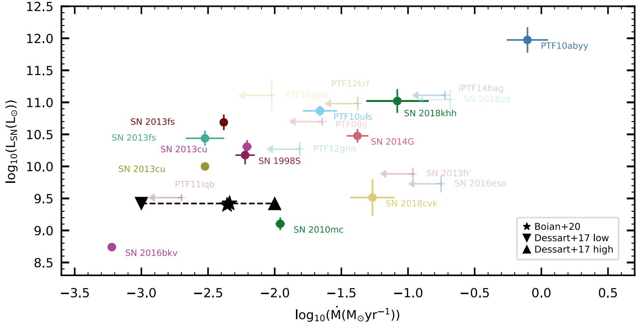
Figure 6. The SN luminosity and mass-loss rate derived by Boian & Groh (2020) for a sample of 17 SNe compared to the best model of SN 2023ixf (black). Upper limits on mass loss are shown with semitransparent markers and arrows, while determined values are solid. We determine a scaled mass-loss rate of \dot{M} \approx 4.5 \times 10^{-3} M_{\odot} \text{ yr}^{-1} and a scaled luminosity of L \approx 2.6 \times 10^9 L_{\odot} from the models of Boian & Groh (2019; with slight variation due to different surface abundances), which we plot as black stars. In practice, these are located at virtually the same location on this plot. We also include the mass-loss rates of the r1w4 and r1w6 models of Dessart et al. (2017) ( \dot{M} = 10^{-3} M_{\odot} \text{ yr}^{-1} , and \dot{M} = 10^{-2} M_{\odot} \text{ yr}^{-1} , respectively), which are shown as black triangles. Dessart et al. (2017) does not explore variations in luminosity, and we therefore use the luminosity derived from Boian & Groh (2019) solar abundance models and do not scale the mass-loss rates. The mass-loss rate of SN 2023ixf is in line with the lower end of the range of mass-loss rates in this sample.
