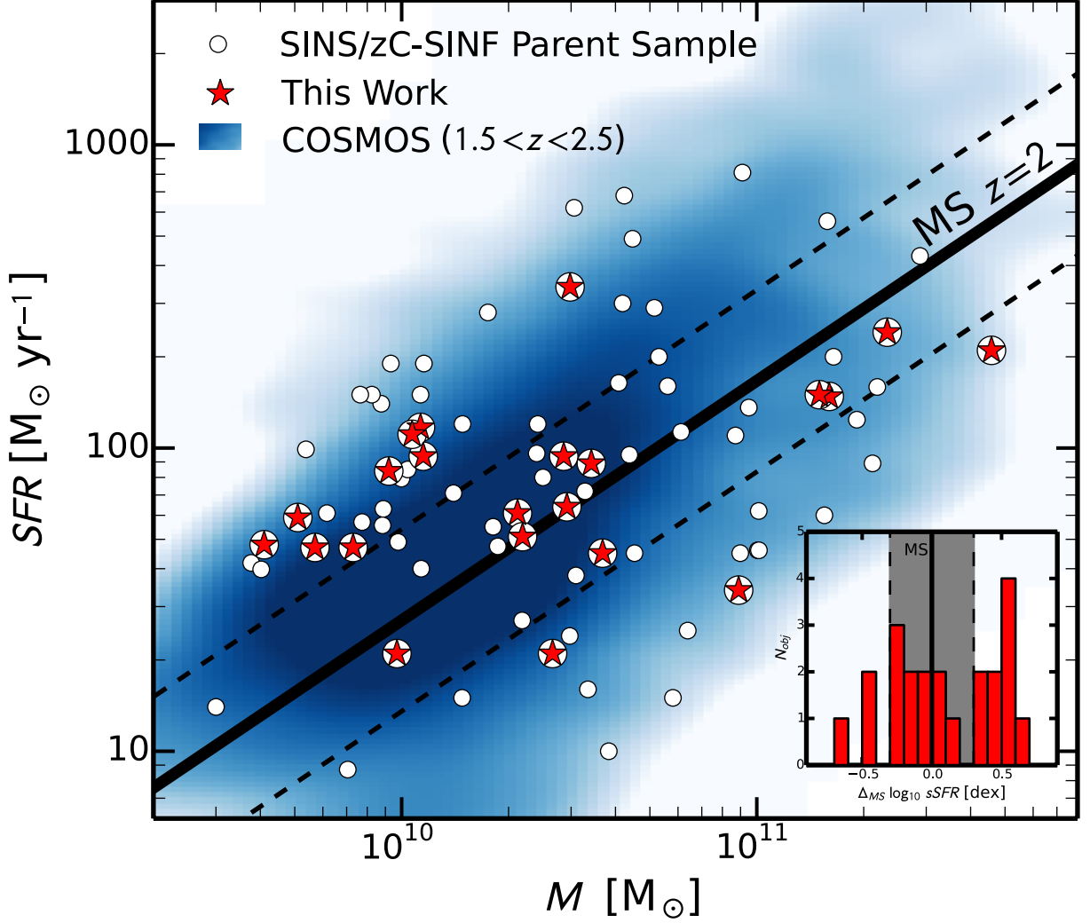
Fig. S1. Location of our sample on the z\sim 2 star-forming main sequence. The black solid line shows the main sequence and dashed lines indicate its 0.3 dex scatter. The white circles show the SINS/zC-SINF parent sample, the red stars are our sample, and the blue shaded regions shows the distribution of \sim 6000 SFGs from the COSMOS survey (58) in the redshift range 1.5 < z < 2.5 . The inset shows the distributions of the offsets in specific SFR from the main sequence (in logarithmic units). The most massive galaxies in our sample are about 0.44 dex below the main sequence, with 4 out of 5 less than 0.4 dex and one at 0.7 dex, consistently with our result that the quenching process is already under way in the cores of these galaxies.
