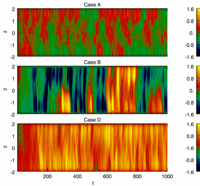
Fig. 3.— Space-time diagrams of average azimuthal field. The horizontally averaged value of B_y is plotted as a function of z and t . The three panels refer to cases A, B and D, with zero net flux and different aspect ratios. The diagram for case D covers the second half of the simulation, the diagram for the full simulation length is shown in Fig. 6. The corresponding values of the plasma \beta are \gtrsim 1 .
