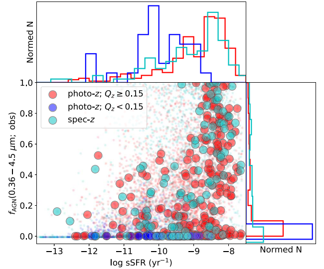
Figure 2. \log sSFR vs. f_{AGN}(0.36-4.5 \mu m; obs) for all the XMM-SERVS sources. Galaxies with cataloged M_* < 3 \times 10^9 M_\odot are marked with large points. Distributions of \log sSFR and f_{AGN}(0.36-4.5 \mu m; obs) are shown in the top and right panels, respectively. Sources whose redshifts are photo- z s with Q_z \geq 0.15 (i.e., the large red points) are removed from our sample. The photo- z quality cut only retains sources with small sSFR and near-zero f_{AGN}(0.36-4.5 \mu m; obs) .
