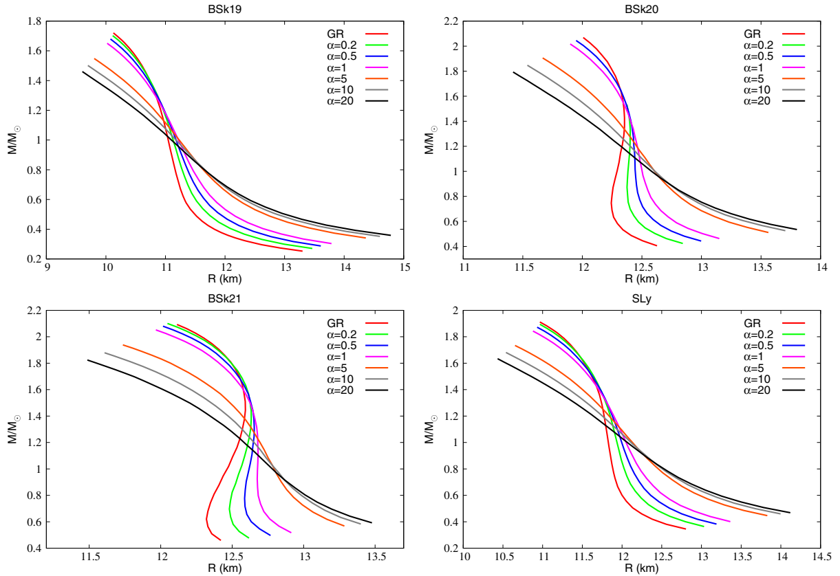
FIG. 2. M - \mathcal{R} diagrams for different EoS (labeled in the top of each panel) and quadratic form f(R) = R + \alpha R^2 . For each EoS the maximal central density is determined by the condition \rho_c - 3p > 0 (see text). The classical TOV solution is also reported. The values of \alpha are in the modulus.
