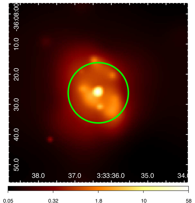
Figure 1. X-ray image of the central 1 arcmin \times 1 arcmin region of NGC 1365 in the 0.3–3 keV energy range (from ObsIDs 13920/1), showing the extent of the diffuse starburst emission and the aperture adopted (green circle, 10 arcsec radius). An adaptive smoothing has been applied following the same criteria of Wang et al. (2009).
