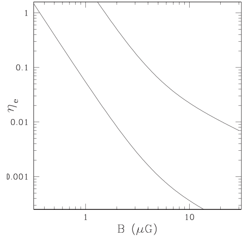
Figure 5. Electron acceleration efficiency versus magnetic field downstream in the shock in A115. Lines represent efficiencies evaluated for re-accelerated electrons with p_{\text{min}}/m_e c = 20 (top) and 200 (bottom) and \delta_{\text{inj}} = 3.8 .
