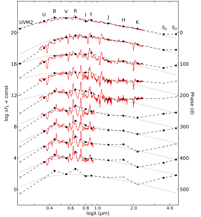
Fig. 6. Evolution of the SED (black dots and dashed lines) before day 500, overplotted with blackbody fits to the V , I , J , H , and K photometry (black dotted lines) and the observed (interpolated; Sect. 3.1) spectra (red solid lines). Fluxes based on extrapolations or interpolations over more than 25 days are shown in shaded colour.
