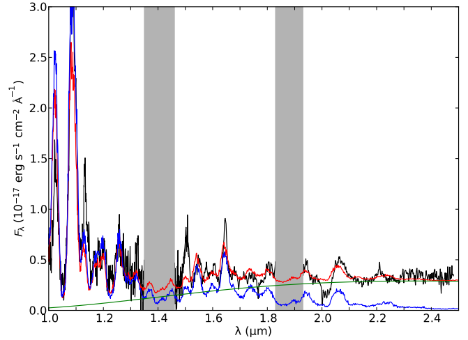
Fig. 21. Observed zJ and HK spectra at days 198 and 206 (black) compared to NIR spectra for the preferred model (12F, red) and model 12E (blue), which differs only in that \tau_{\text{dust}} = 0 . The observed spectra were flux calibrated with the interpolated observed J , H , and K magnitudes at day 200 and we also show the dust emission component for the preferred model (green).
