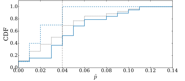
Fig. 2. J1505+0326: The distribution of the de-biased polarisation fraction p . The dot-dashed vertical line marks the median of the distribution. The blue dashed line shows the distribution of \hat{p} during the non-rotating phases and the solid one that during the rotating phases. The black dotted line corresponds to all the measurements.
