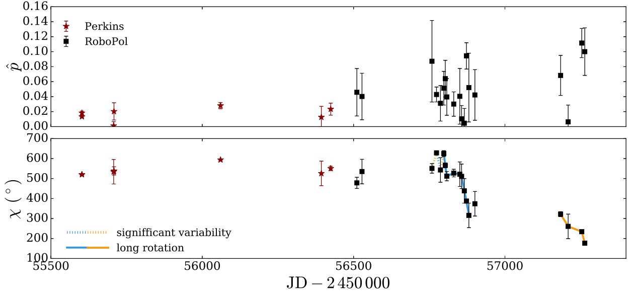
Fig. 1. J1505+0326: De-biased polarisation fraction p and adjusted EVPA ( \chi ) as a function of time. The coloured lines mark periods of significant monotonous – within the uncertainties – EVPA evolution. Solid lines mark periods of long rotations (i.e. at least three sequential data points and angle larger than 90^\circ ). Blue and orange connecting lines are used alternatively to ease reading.
