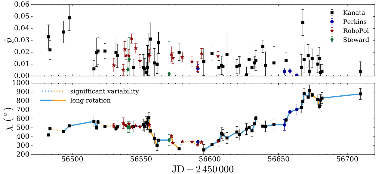
Fig. 12. J0324+3410: A zoom on the region of the largest potential rotations.
