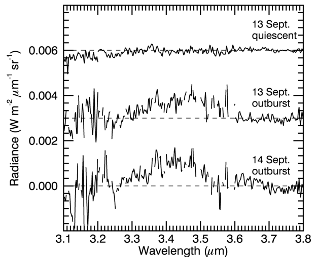
Figure 15. VIRTIS-H spectra of the 3.4 \mu\text{m} band observed on 2015 September 13 and 14. Labelled outburst spectra correspond to 13 September 13.712–13.792 h UT (middle) and 14 September 18.863–18.897 h UT (bottom). The spectrum labelled quiescent is the average of 850 acquisitions acquired before the September 13 outburst. The dust continuum emission has been removed. Outburst spectra include the contribution of the background coma, which is low. The outburst and quiescent September 13 spectra have been shifted by +0.003 and +0.006, respectively, in radiance units. Spectral channels found to be much more noisy than nearby channels have been removed.
