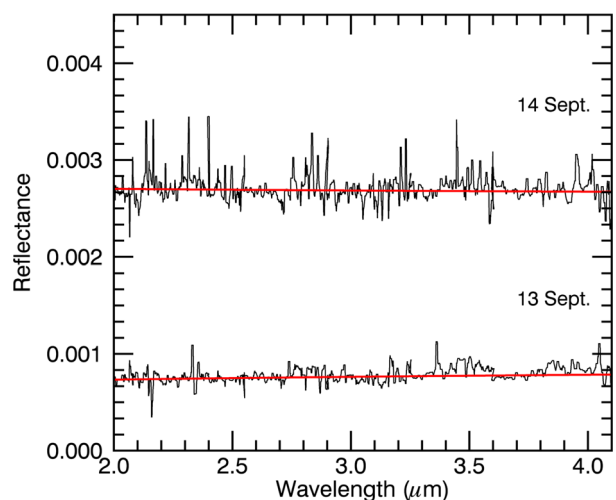
Figure 13. Reflectance spectra of outburst ejecta. Acquisitions 921–1051 (13 September 13.712 46–13.986 18 h UT) and 661–691 (14 September 18.905 40–18.968 21 h UT) were considered. The September 14 spectrum has been shifted vertically by +0.002 . A median smoothing with dimension 6 has been applied. The reflectance is defined by R(\lambda) = \pi I(\lambda) r_h^2 / F_{\odot}(\lambda) , where I(\lambda) is the measured radiance after removing the thermal radiation. The solid red line is the fitted reflectance over the full VIRTIS-H spectrum.
