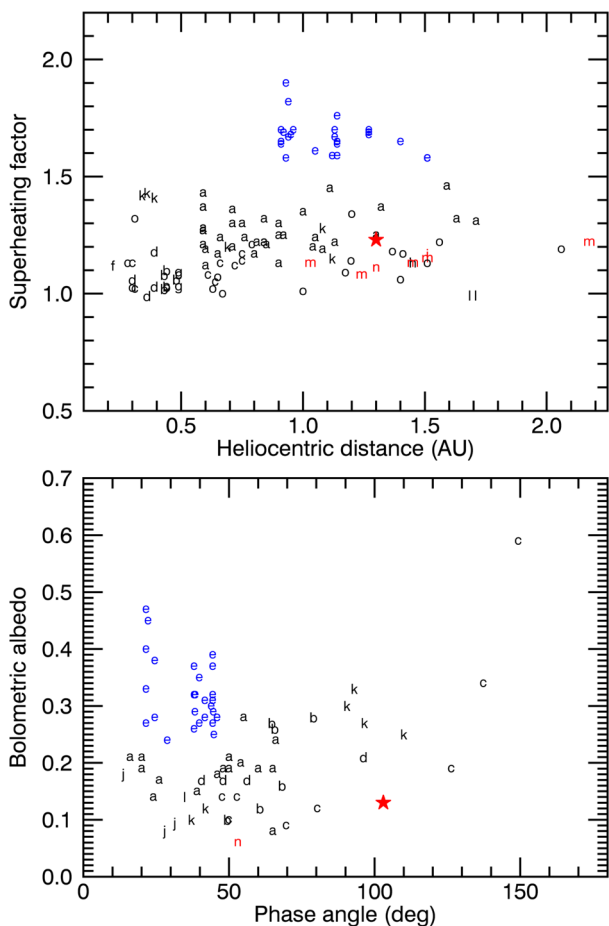
Figure 16. Superheat factor S_{\text{heat}} (top) and bolometric albedo A (bottom) measured in comets (letters) compared to 67P values for the quiescent coma at 1.3 au from the Sun (this work). Letters correspond to comets: (a) 1P/Halley, (b) C/1975 N1 (Kobayashi-Berger-Milon), (c) C/1980 Y1 (Bradfield), (d) C/1989 X1 (Austin), (e) C/1995 O1 (Hale-Bopp), (f) C/1985 K1 (Machholz), (g) 23P/Brorsen-Metcalf, (h) C/2007 N3 (Lulin), (i) 9P/Tempel 1, (j) C/2009 P1 (Garradd), (k) C/1996 B2 (Hyakutake), (l) C/2012 K1 (PAN-STARRS), (m) Jupiter-family comets 69P/Taylor, 4P/Faye, 19P/Borrelly, 55P/Tempel-Tuttle, 24P/Schaumasse, (n) 103P/Hartley 2, (o) long-period comets reported in Sitko et al. (2004). Other measurements are from Gehrz & Ney (1992), Gicquel et al. (2012), Mason et al. (1998), Mason et al. (2001), Meech et al. (2011), Sitko et al. (2013), Woodward et al. (2011), Protospapa et al. (2014), Woodward et al. (2015). Blue colours are used for comet Hale-Bopp. A red colour is used for Jupiter-family comets.
