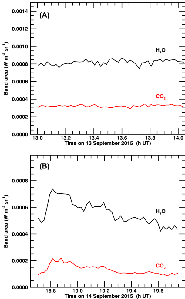
Figure 14. Temporal evolution of the areas of the H 2 O 2.7 \mu\text{m} and CO 2 4.26 \mu\text{m} bands at the time of the September 13 (A) and September 14 (B) outbursts. The time resolution is \sim 70 s. The spectral ranges used for computing the band areas are 2.55–2.74 and 4.20–4.35 \mu\text{m} , for H 2 O and CO 2 , respectively.
