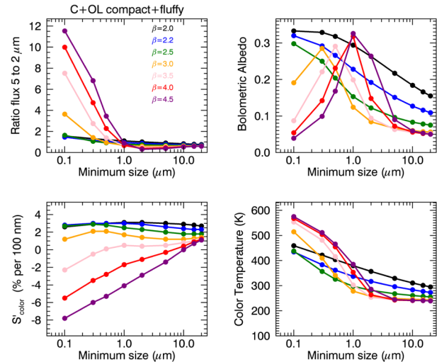
Figure 11. Results for relative fractions of 25 percent of fractal aggregates and 75 percent of moderately porous carbon/olivine mixtures ( P_{\text{max}} = 0.5 ). See captions to Figs 8 and 9. The model parameters are q_{\text{frac}} = 0.7 , a_{\text{unit}} = 100 nm, D = 2.5 for compact grains and D = 1.7 for fluffy grains. The Mg:Fe content of olivine is 50:50.
