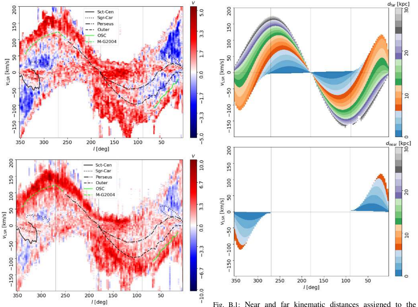
Fig. B.1: Near and far kinematic distances assigned to the 3^\circ \times 20^\circ \times 1.29 \text{ km s}^{-1} tiles used to construct the l - v diagrams in Fig. 1. These results correspond to the solutions of Eq. B.3 using the rotation curve presented in Reid et al. (2019).
