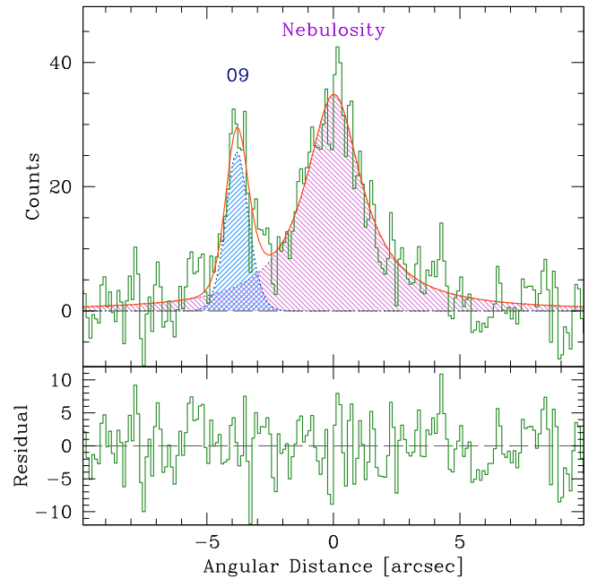
Figure 3. Example of our deblending procedure on a 3 pixel slice of the 2D long-slit spectrum centred at \lambda = 5500 \text{ \AA} . Top panel: spatial profile of the two spectra (green line). The contributions of PKS 2155–304_09 and of the PKS 2155–304's nebosity were deblended performing a simultaneous fit with a Gaussian and a Lorentzian function, respectively (blue and purple shaded areas). The result of the fit is also shown (orange line). Bottom panel: residual spectrum.
