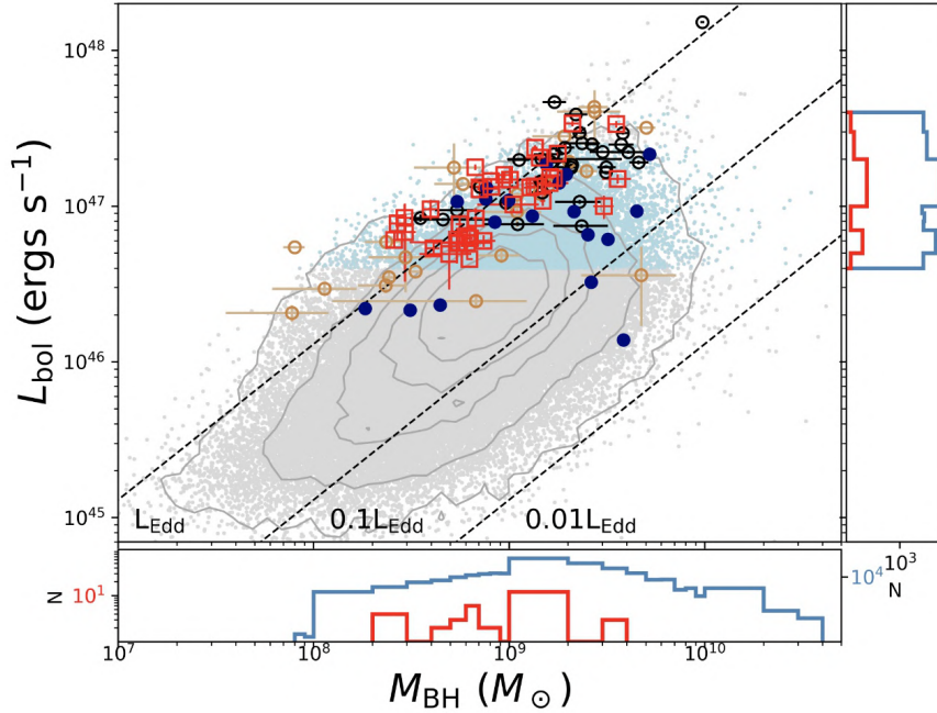
Fig. 1 Bolometric luminosities and black hole masses of a compilation of 6.0 \lesssim z \lesssim 7.6 QSOs (red, black, and brown symbols) compared with the SDSS lower-redshift ( 0.40 < z < 2.1 ) sample (grey dots). The light blue dots represent a sub-sample from the SDSS lower redshift survey with bolometric luminosity comparable to the highest-redshift sample presented by [1] (red). The right-hand and bottom histograms show the comparison of the luminosity and black hole mass distributions, respectively, in the two aforementioned samples, with the same colour-coding. The figures show that a large number of high-redshift QSOs are located close to (or above) the line of Eddington luminosity (upper dashed line). Figure is taken from [1]. ©AAS. Reproduced with permission.
