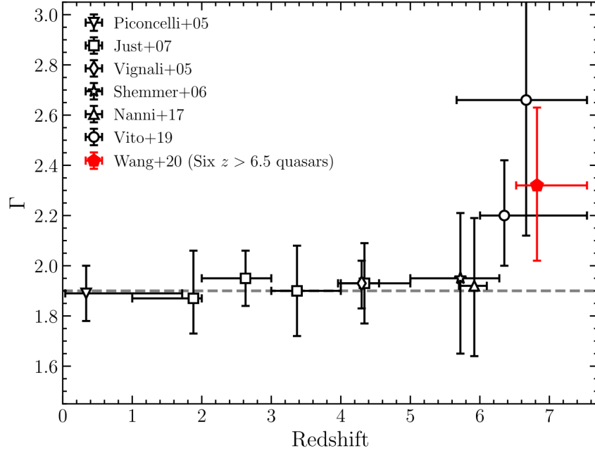
Fig. 12 Average photon index of optically selected QSOs as a function of redshift. From [132]. © AAS. Reproduced with permission.
