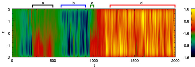
Figure 6. Space-time diagram of the average azimuthal field for case D. The horizontally averaged value of \hat{B}_y is plotted as a function of z and t . The diagram covers the full simulation length of 2000 time units. Above the diagrams we have marked four time intervals, denoted by the letters a, b, c, and d, during which we have alternatively low and high states. The time-averaged vertical profiles of azimuthal field shown in Figure 7 refer to these four time intervals.
