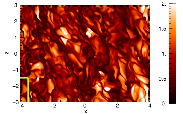
Figure 4. Typical temperature plenum at the upper boundary of the computational box for case D with zero net flux and the largest aspect ratio. The green rectangle in the lower left corner of the figure shows the extent of the computational grid for case A.
