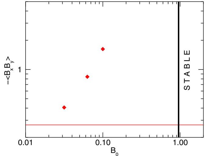
Figure 11. Box and time-averaged values of the Maxwell stresses for cases E–G as a function of the initial vertical field strength B_0 . The horizontal line corresponds to the average stress value for case D with zero net flux in the high state. The vertical line shows the linear stability boundary for a state with constant density.
