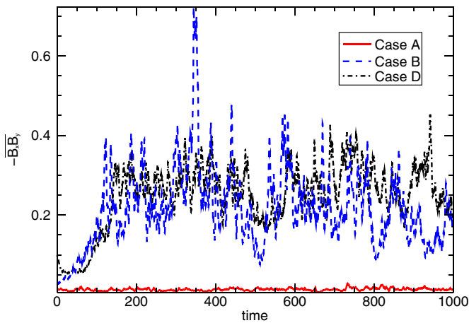
Figure 2. Time histories of the Maxwell stresses averaged over the computational box for the cases A, B, and D with zero net flux and different aspect ratios. The time history for case D covers the second half of the simulation, the full time history for this case is shown in Figure 5.
