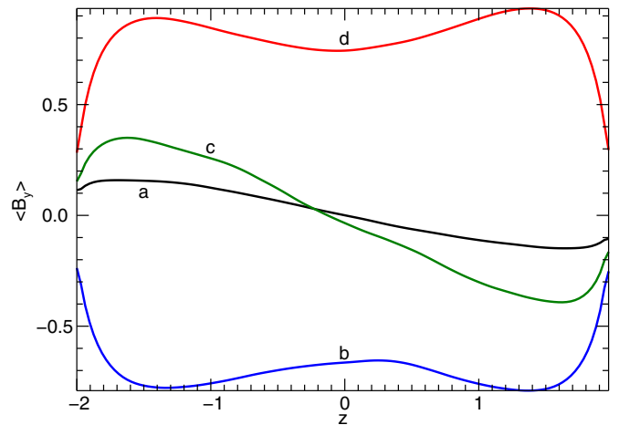
Figure 7. Vertical profile of the time-averaged azimuthal field as functions of z . The four curves refer to the four time intervals—a, b, c, and d—marked in Figure 6, for which we have alternatively low and high states.
