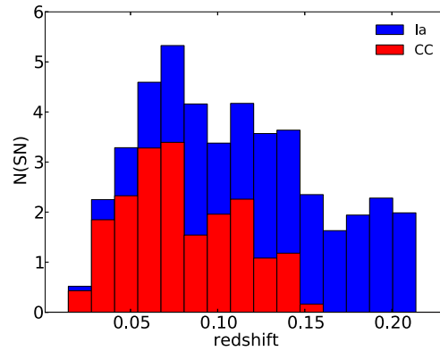
Figure 7. Simulated numbers of core-collapse and Type Ia SNe predicted to be detected within the sky survey area and their redshift distribution. See Section 5.1 for details.
