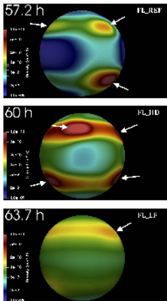
Fig. 9. Maps of particle number density in log scale close to the stellar surface after about 60 h of evolution for runs FL-REF (upper panel), FL-HD (middle panel), and FL-LF (lower panel). The high-density regions (pointed at by white arrows) correspond to accretion columns impacting onto the stellar surface. Runs FL-REF and FL-HD exhibit clear hotspots, whereas in run FL-LF, the matter is more diffused and the contrast in density is weaker.
