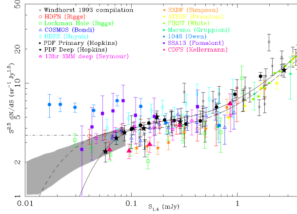
Figure 2: The Euclidean normalised differential radio source counts at 1.4 GHz (taken from Norris et al., 2013; Hopkins et al., 2003). The curves are alternative polynomial fits. The horizontal dot-dashed line represents a non-evolving population in a Euclidean universe. The shaded region shows the prediction based on fluctuations due to weak confusing sources ( P(D) analysis: Condon et al., 1974; Mitchell & Condon, 1985).
