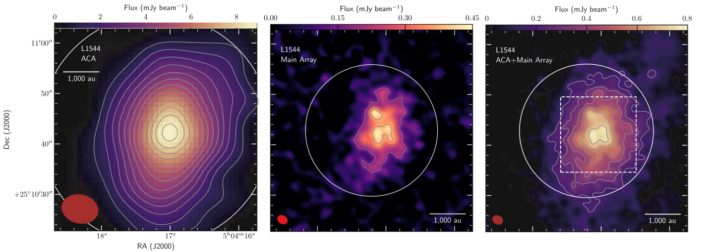
Figure 1. 1.3 mm dust continuum emission toward L1544 as seen by: (left) the ACA, with contours starting at 5\sigma (with \sigma = 0.21 mJy beam ^{-1} ) in steps of 3\sigma ; (center) the 12 m array only, with contours starting at 5\sigma (with \sigma = 34 \mu Jy beam ^{-1} ) in steps of 3\sigma ; and (right) combined ACA+12 m array, with contours starting at 5\sigma (with \sigma = 36 \mu Jy beam ^{-1} ) in steps of 3\sigma . The white dashed square is the area shown in Figure 2. The white circles in the three panels represent the corresponding 50% primary beam response. The red ellipses in the bottom left of the three panels are the synthesized beams.
