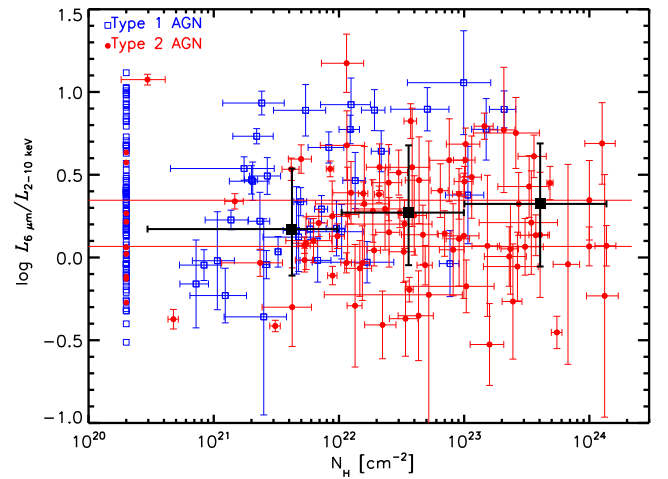
Figure 10. Mid-IR to X-ray luminosity ratio (in logarithmic units) versus the line-of-sight X-ray absorption. For clarity, we have arbitrarily assigned a column density of 2 \times 10^{20} \text{ cm}^{-2} to the unabsorbed objects. Large filled squares and their vertical error bars are the median and 16 and 84 percentiles in different column density intervals indicated with the horizontal error bars.
