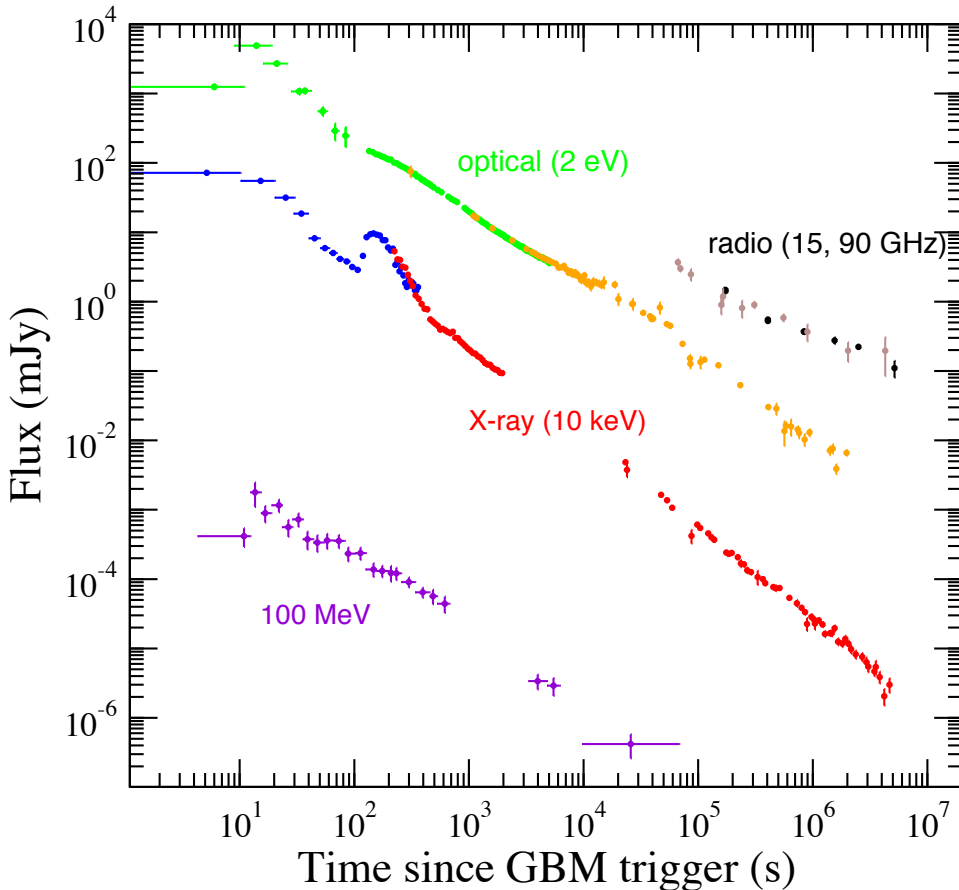
Figure 4: Example of a GRB afterglow in different spectral ranges. The data reported are for GRB 130427A afterglow (Panaitescu et al. 2013). (Figure courtesy of Alin Panaitescu).
