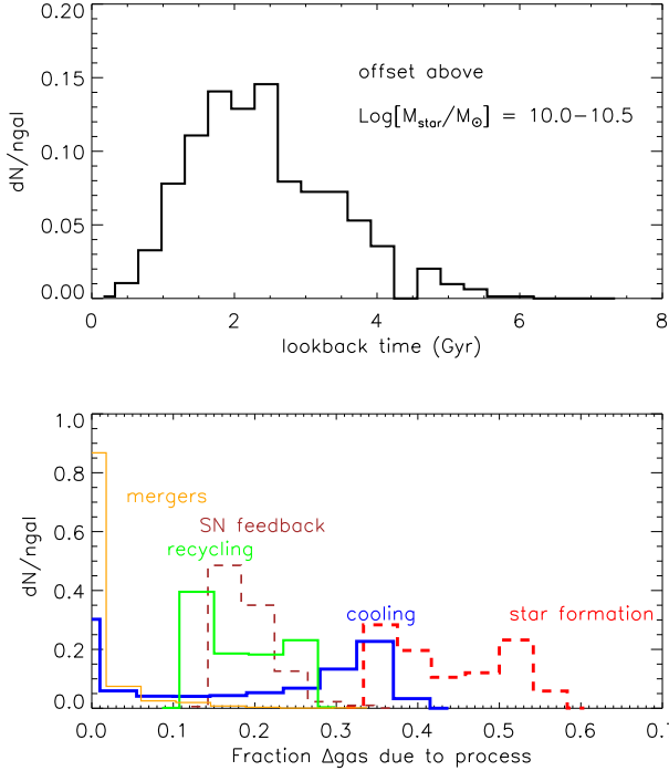
Figure 9. The top panel shows the distribution of the lookback times when the main progenitor crosses (for the first time going backward in time) the best-fit relation found for model galaxies at z = 0 . The bottom panel shows the fractional contributions of different physical processes to the absolute variation of cold gas in model galaxies, between the crossing time defined above and today. Contributions from processes that cause negative/positive variations of the cold gas mass are shown with dashed/solid lines. Increasing line thickness is used for stellar feedback, star formation (that cause negative variations of cold gas) and mergers, recycling and cooling (that lead to positive variations of cold gas).
