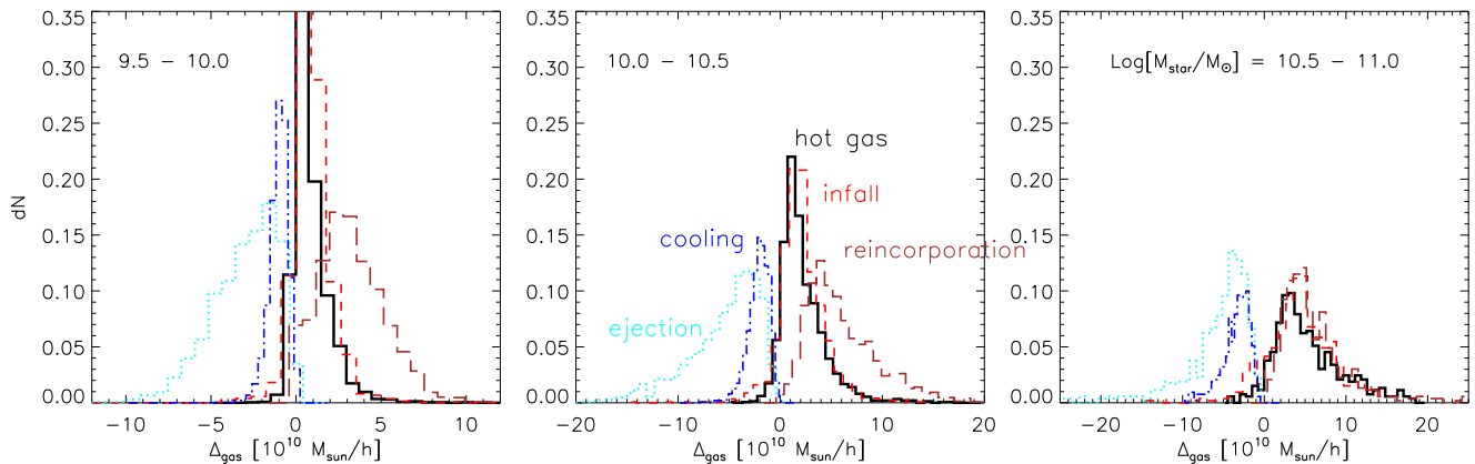
Figure 11. Variations of hot gas (black solid histograms), cosmologically infalling gas (dashed red), ejected gas (dotted cyan), cooling gas (dot-dashed blue) and re-incorporated gas (long-dashed brown), between the time corresponding to the last maximum metallicity value and the present time. The three panels correspond to different galaxy stellar mass bins, as indicated in the legend.
