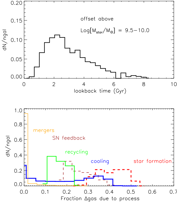
Figure A1. As in Fig. 9, but for galaxies with stellar mass between \log(M_{\text{star}}/M_{\odot}) = 9.5 and \log(M_{\text{star}}/M_{\odot}) = 10 .
