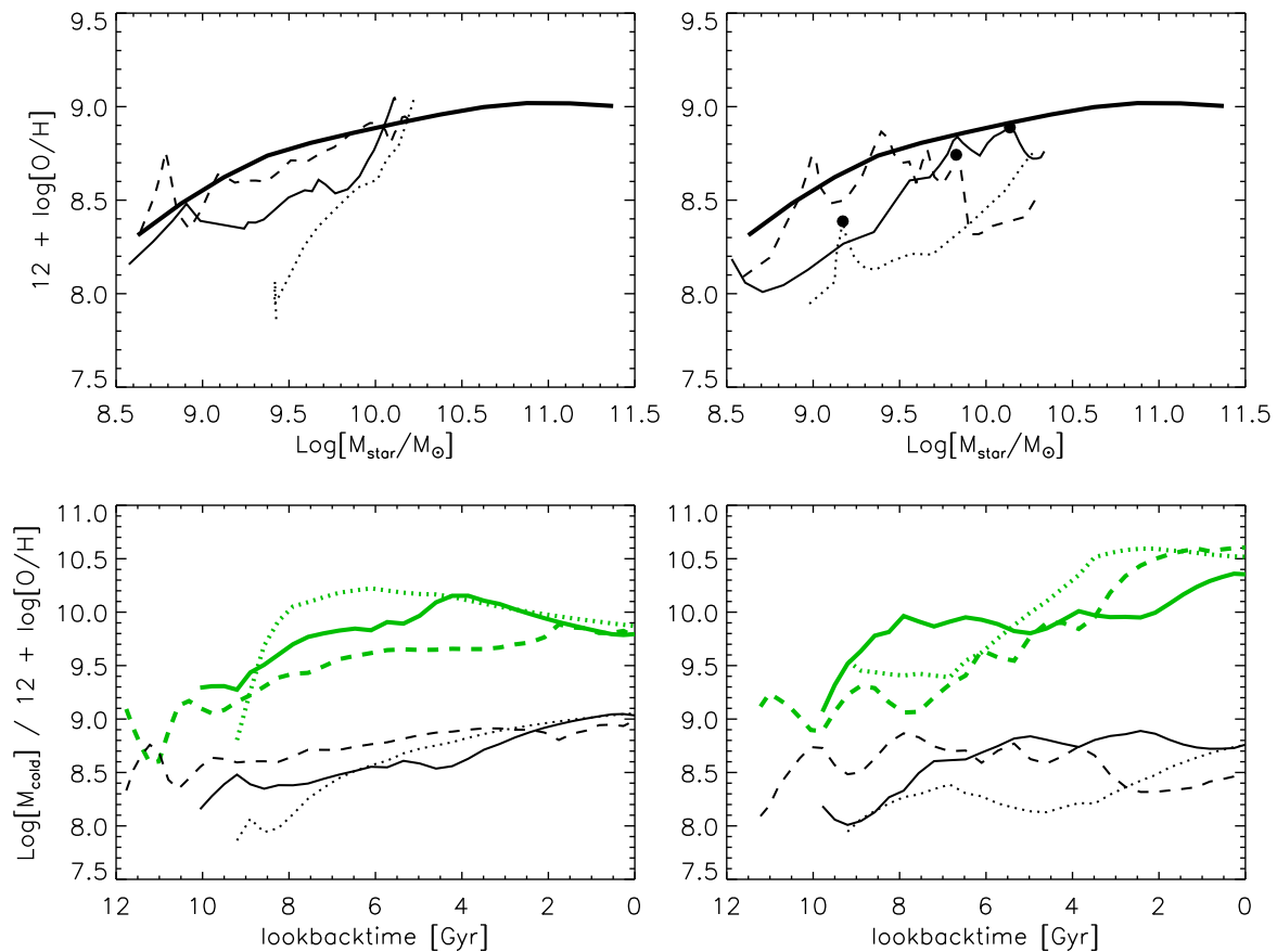
Figure 7. Top panels show the trajectories of a few example galaxies in the stellar mass - gaseous metallicity plane. Left and right panels are for galaxies offset above and below the mass-metallicity relation, respectively. Dashed and dotted lines correspond to example galaxies whose trajectories are relatively close or distant from the predicted relation at z=0 (thick solid line) for a significant fraction of the galaxy’s lifetime. Solid lines correspond to intermediate cases (the most frequent among the model galaxies analysed - see text). The bottom panels show the corresponding evolution of the cold gas mass (thick green lines) and gaseous metallicity (black lines). The filled circles in the top right panel mark the first metallicity maximum, going backwards in time, identified for each model galaxy (this will be used later in our analysis).
