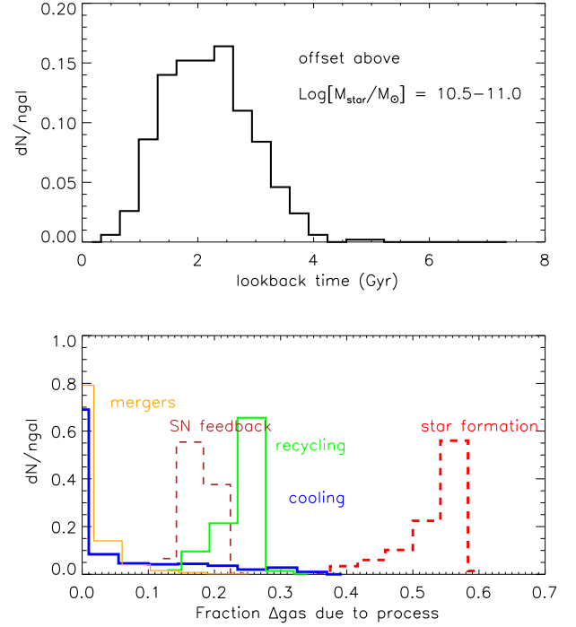
Figure A2. As in Fig. 9, but for galaxies with stellar mass between \log(M_{\text{star}}/M_{\odot}) = 10.5 and \log(M_{\text{star}}/M_{\odot}) = 11 .
