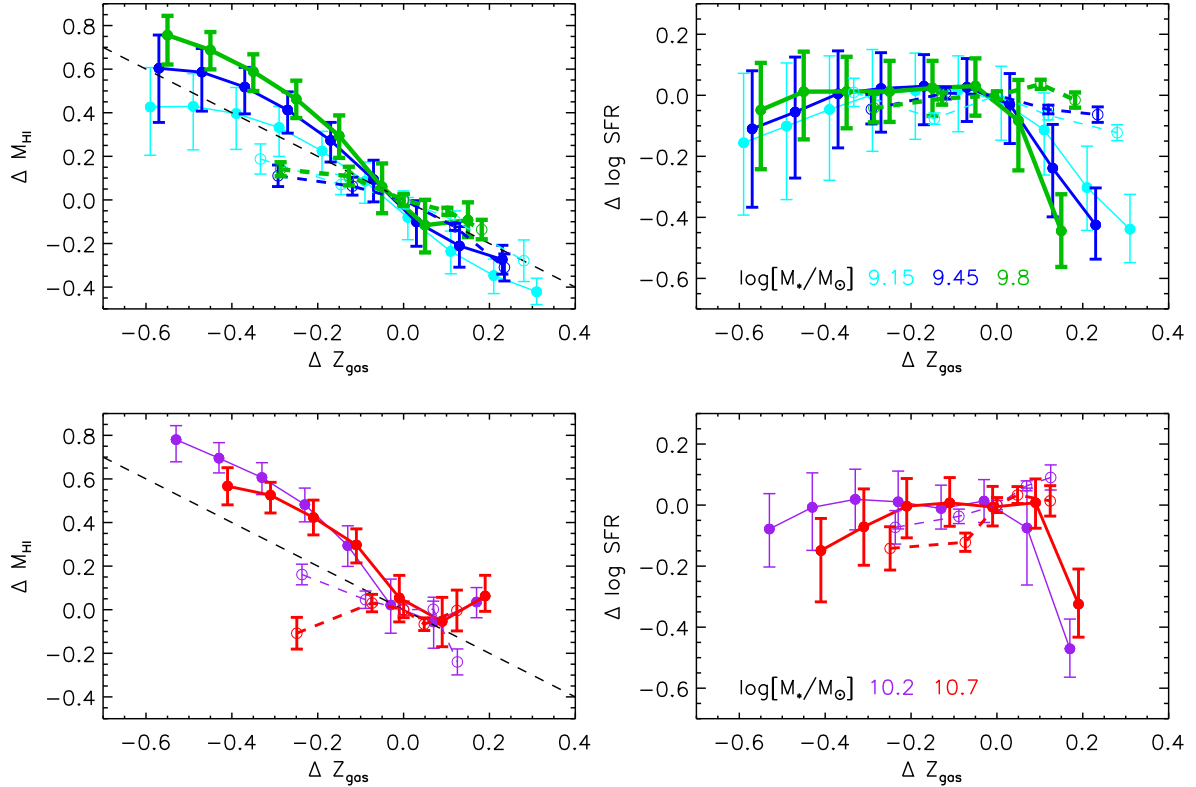
Figure 6. Differences of HI mass (left panels) and star formation rate (right panels) as a function of the differences in metallicity from the value of the same quantities on the mass-metallicity relation. Top and bottom panels show different stellar mass bins, with model predictions shown as filled symbols connected by solid lines and observational estimates by (Brown et al. 2018) marked by open circles connected by dashed lines. In all panels, the line thickness increases with increasing galaxy stellar mass.
