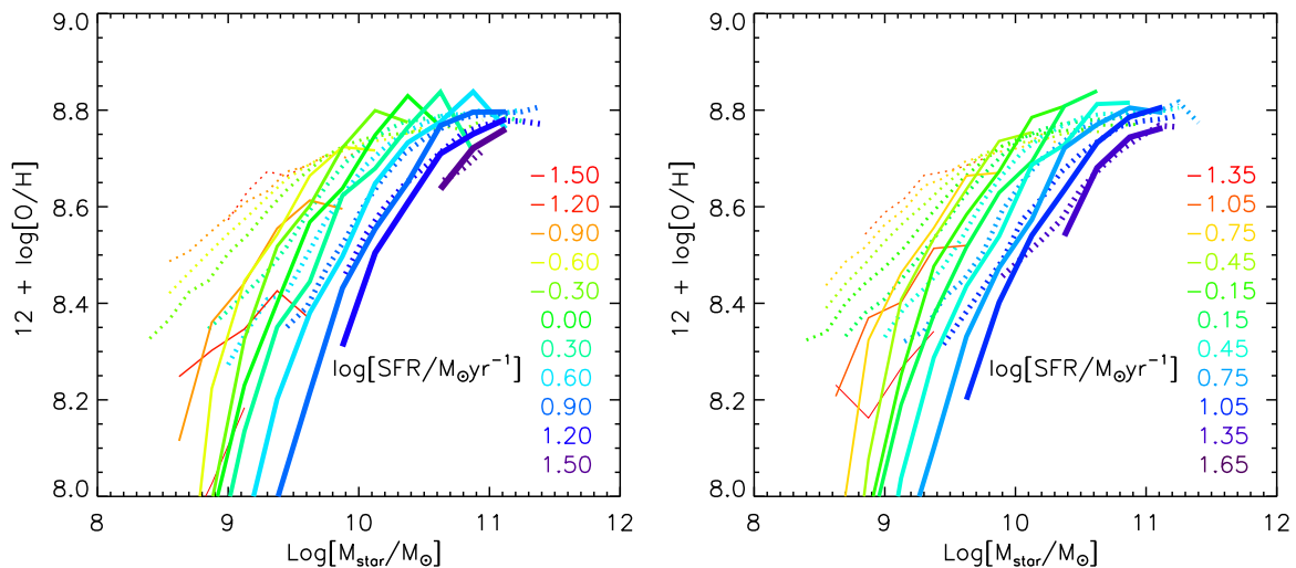
Figure 4. Cold gas metallicity as a function of galaxy stellar mass, for bins of galaxies with different star formation rates as indicated in the legend. Dotted lines show observational measurements by Curti et al. (2020), while solid lines show predictions based on our reference model. The line thickness increases with increasing values of the star formation rate. A constant vertical shift of -0.22 has been applied to all model predictions. These have not been convolved with observational uncertainties. When this is done, the dependence on star formation rates disappears for the 5-6 bins with lowest star formation rates, while the trends shown for bins with larger star formation rates are not significantly affected.
