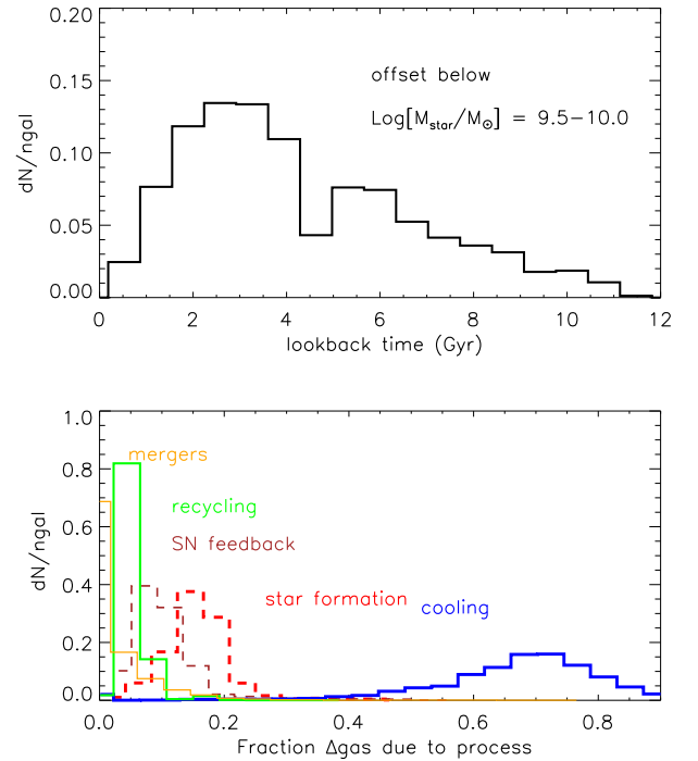
Figure A3. As in Fig. 10, but for galaxies with stellar mass between \log(M_{\text{star}}/M_{\odot}) = 9.5 and \log(M_{\text{star}}/M_{\odot}) = 10 .
