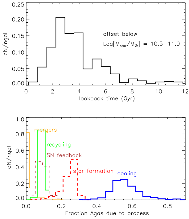
Figure A4. As in Fig. 10, but for galaxies with stellar mass between \log(M_{\text{star}}/M_{\odot}) = 10.5 and \log(M_{\text{star}}/M_{\odot}) = 11 .
