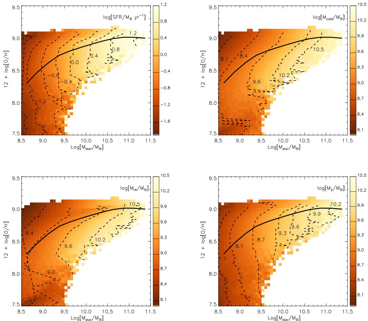
Figure 2. As in Fig. 1, but colour-coded as a function of the median of the quantity indicated on the top right of each panel. The black solid line shows the median mass-metallicity relation obtained for all star-forming model galaxies considered (see text for details). Dashed lines show the location of star-forming galaxies whose median value of the quantity indicated on the top-right of the panel is close (within 0.3 dex) to that indicated close to each line.
