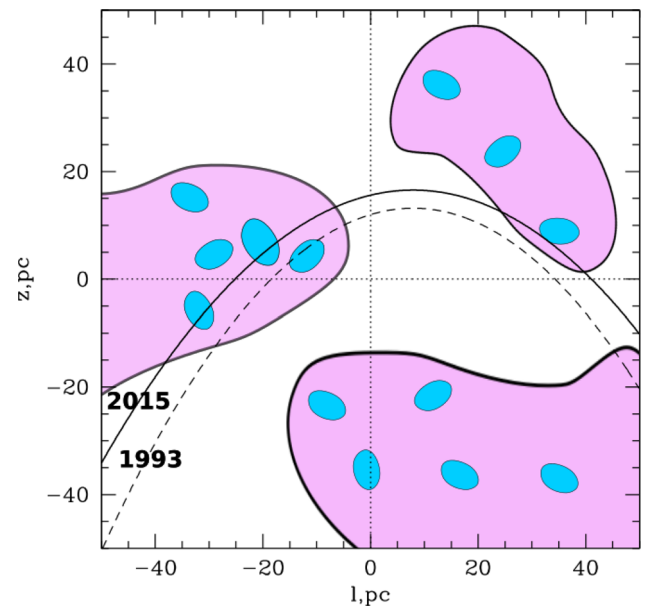
Figure 3. Sketch of a short outburst scenario for the outburst that happened \sim 110 yr ago, assuming that the primary source is at (0,0). This is a view on the Galactic Center region from the Galactic pole, with the galactic longitude l along the horizontal axis, and the line-of-sight distance z along the vertical axis. The dashed and solid lines correspond to the position of the ‘light-front’ in 1993 and 2015, respectively. The distance along the line of sight between the illuminated regions is given by \sim \frac{\partial z}{\partial t}(t_2 - t_1) , where t_2 - t_1 \sim 22 yr (see text). For regions close to primary source in projection, the value \frac{\partial z}{\partial t} \sim 0.5c . This value increases with projected distance from the primary source.
