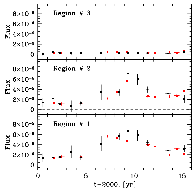
Figure 5. Light curves of reflected emission for selected regions. Left: three regions used for the analysis, superposed on to the Chandra map. Regions 1 and 2 are located within the molecular complex bright in reflected emission. Region 3 is a test region where reflected emission is faint. Right: light curves for regions 1, 2 and 3 (from bottom to top). Red and black points correspond to XMM-Newton and Chandra observations, respectively. The duration of the peaks sets an upper limit on the duration of the outburst. Even for an extremely short outburst the finite spatial extent of each cloud along the line of sight broadens the peak. For instance, for a cloud with size of 1 pc, the minimum duration of the observed outburst, given \frac{\partial z}{\partial t} \sim 0.75c is 4.3 yr.
