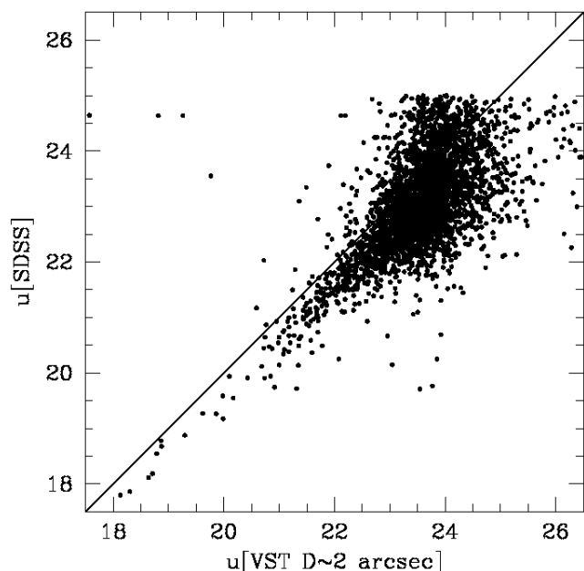
Fig. 3. Comparison between the u magnitudes of SDSS and our VST data for the star sample using a different aperture for the photometry of the VST data.
