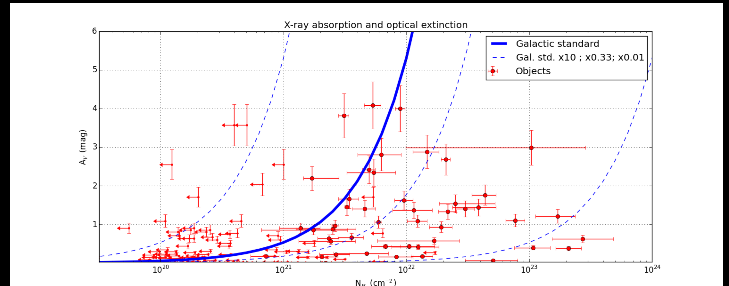
Figure 6: Dust-to-gas ratio for the BUXS type-1 sample. We represent here the plot of A_{\text{V}} vs N_{\text{H}} for our objects, with the 68 per cent confidence errors. If we can only derive a 68 per cent confidence upper limit to the N_{\text{H}} it is indicated with an arrow. The solid line represent the Galactic ratio and the dashed lines represents 10 times higher and 3 and 100 times lower than the Galactic ratio.
