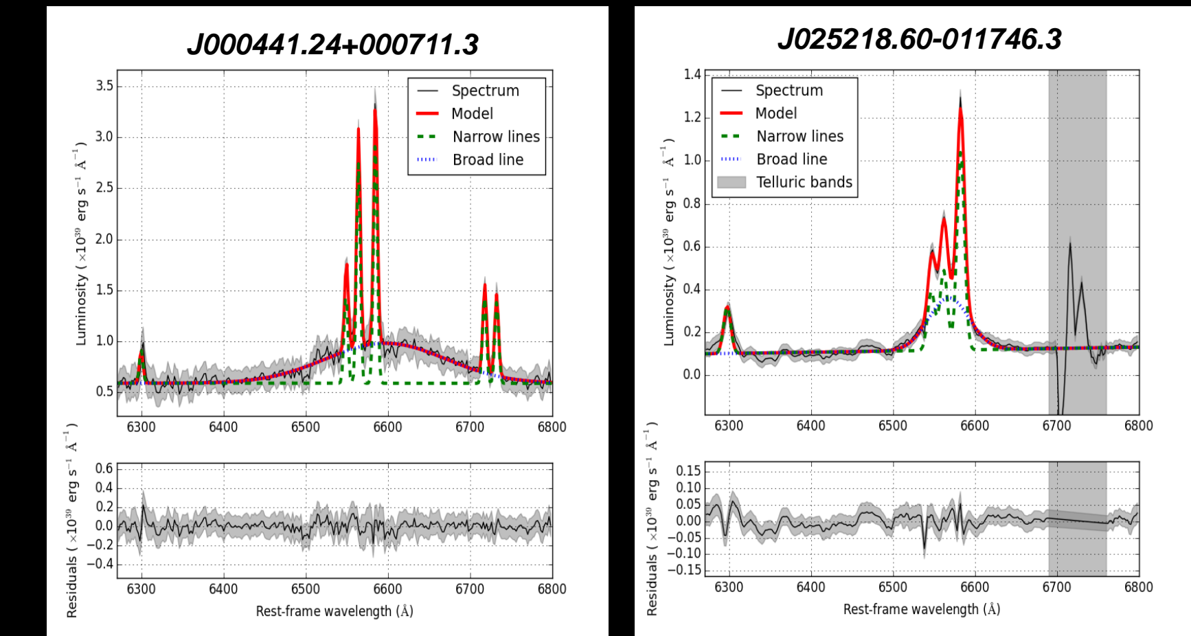
Figure 4: Spectrum of the nucleus of J000441.24+000711.3 (left) and J025218.60-011746.3 (right). Top: H \alpha region and its decomposition in narrow and broad lines. The emission lines are fitted with gaussian functions and the local continuum with a power law. Bottom: Residuals of the fits. Errors are 68 per cent confidence.
