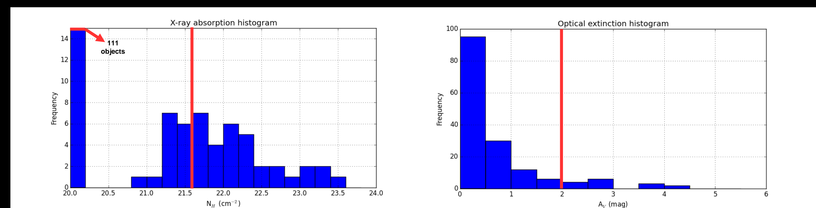
Figure 5: Histogram of X-ray absorption in terms of N_{\text{H}} (left) and histogram of optical extinction in terms of A_{\text{V}} (right) for the BUXS type-1 sample. We use the limit of \log(N_{\text{H}}) = 21.6 \text{ cm}^{-2} (with a red line), the equivalent of A_{\text{V}} = 2 \text{ mag} for a Galactic dust-to-gas ratio (Caccianiga et al. 2008), to divide the sources between X-ray absorbed or not. We also put this limit in the A_{\text{V}} histogram with a red line.
