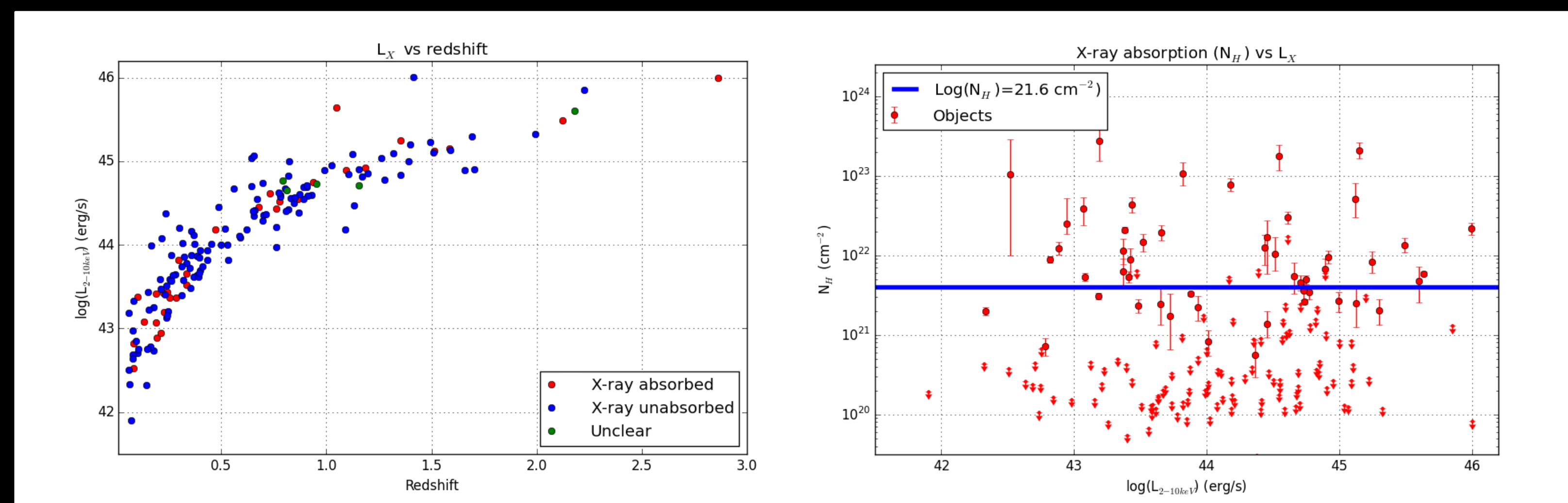
Figure 4: \log(L_{\text{x}}) vs redshift (left) and \log(N_{\text{H}}) vs \log(L_{\text{x}}) plots (right) for the BUXS type-1 sample. The values of the N_{\text{H}} are represented with 68 per cent confidence errors. If we can only derive a 68 per cent confidence upper limit to the N_{\text{H}} it is indicated with an arrow.
