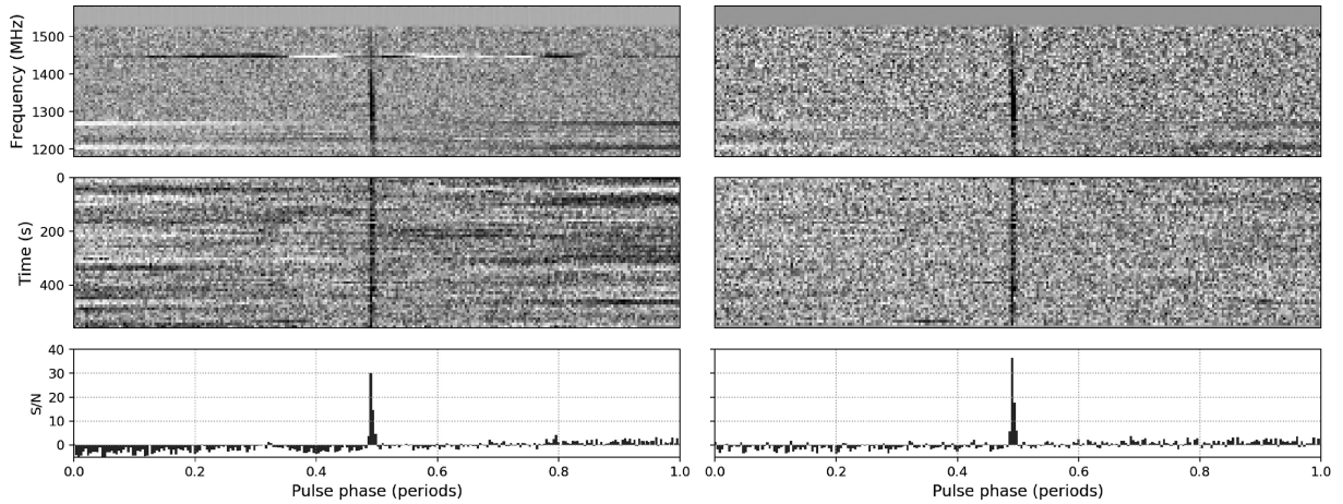
Figure 2. A folded 9-min observation of PSR J0736–6304 ( P = 4.86 s, DM = 19.4 pc \text{cm}^{-3} ) before and after the RFI mitigation algorithms described in Section 2.4 have been applied (left and right columns, respectively). Top: frequency-phase plots, where we have grouped and summed the original 1024 frequency channels into 64 sub-bands for readability. Centre: time-phase plots. Bottom: integrated pulse profiles over the entire observation. In both cases, integrated profiles have been normalized by a factor s\sqrt{N} , where N is the number of unmasked profiles in the cube, and s the standard deviation of unmasked data. The top 150 frequency channels are permanently occupied by telecommunication signals and masked by an RF filter (Keith et al. 2010). The peak S/N of the pulse increases noticeably from 31 to 37. Improving the general quality of candidate plots reduces the probability of genuine pulsars being improperly rejected in the classification stage of a blind search.
