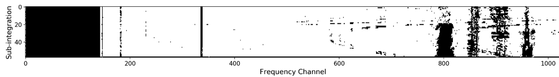
Figure 4. Profile mask determined from the analysis shown in Fig. 3. Each pixel corresponds to a pulse profile, which is part of a given frequency channel ( X -axis) and sub-integration ( Y -axis). Outliers appear in black and the corresponding data are zero-weighted before further processing. Bad frequency channels are successfully flagged in this example. Arc-like patterns are visible, revealing narrow-band interference sources whose frequencies change over a time-scale of \approx 10 s.
