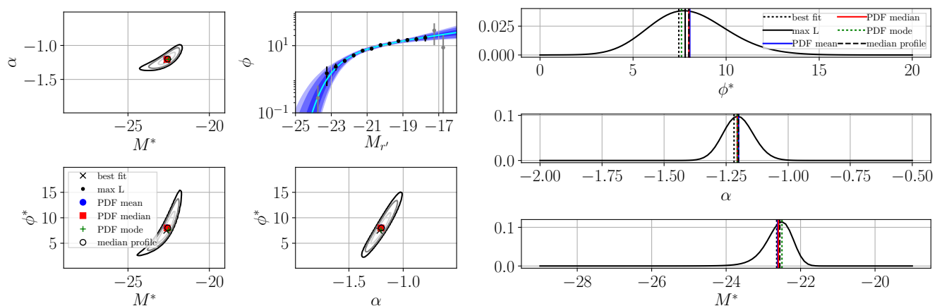
Fig. 15. Illustration of the composite luminosity function fitting procedure for a sample of 121 clusters (general sample in Section 5). Left panels: 2D marginalised likelihoods of the Schechter fit parameters, and associated luminosity profile. The contours show the 68%, 95%, and 99% levels, and the different statistical values are indicated in the legend. Top left: (\alpha, M^*) marginalised over \phi^* ; Top right: Posterior CLF shape, the data points are shown in grey and black, the median profile is drawn in cyan, and the blue shaded regions indicate the 68%, 95%, and 99% c.i.; Bottom left: (\phi^*, M^*) marginalised on \alpha ; Bottom right: (\phi^*, \alpha) marginalised on M^* . Right panels: Probability density functions of the Schechter fit parameters after marginalisation. The lines show the different statistical values, as indicated in the legend. In this sample the different statistical estimators give indistinguishable values.
