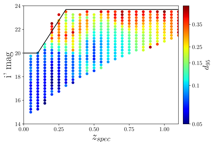
Fig. 5. Photometric redshift dispersion d_{95} , computed as the 95th percentile of |z_{phot} - z_{spec} - bias(z_{spec})| in the ( z, i' mag ) plane. The dots indicate the centres of the \Delta(z, i' mag) = 0.1 \times 0.5 cells used to compute the dispersion (if they contain at least 30 objects). The continuous black line shows the limiting magnitude we impose for the rest of the study.
