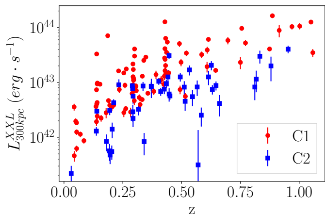
Fig. 1. X-ray luminosity in the [0.5–2]keV band computed in a 300kpc aperture as a function of redshift for the cluster sample used in this study. Red points and blue squares represent clusters classified as C1 and C2, respectively (see text).
