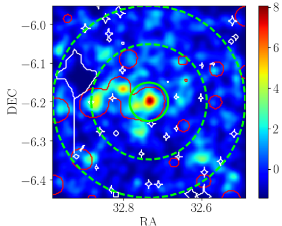
Fig. 6. Example of a density map of a cluster 10 \times 10 Mpc ^2 field, constructed using a Gaussian kernel of width \sigma = 0.1875 Mpc. The colourbar reflects the signal-to-noise ratio. Only galaxies with m < m^* + 3 (or L > 0.06L^* ) are selected and the photometric redshift width depends on the galaxy magnitudes and is taken to ensure 68% completeness. The red contours indicate the structures detected by WAZP, and the white ones show the masked regions. The green inner circle shows 1 Mpc around the cluster X-ray centre and the dashed green lines delimitate the local background field from 3 to 5 Mpc. NB: We can see that this cluster is part of a superstructure.
