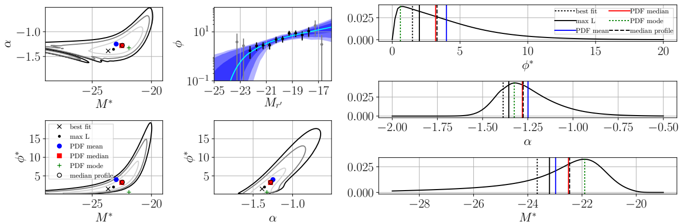
Fig. 16. Illustration of the composite luminosity function fitting procedure as in Figure 15, but for a sample of 26 poor clusters (lowest richness sample in Section 5). In this sample the different statistical estimators give distinguishable values.
