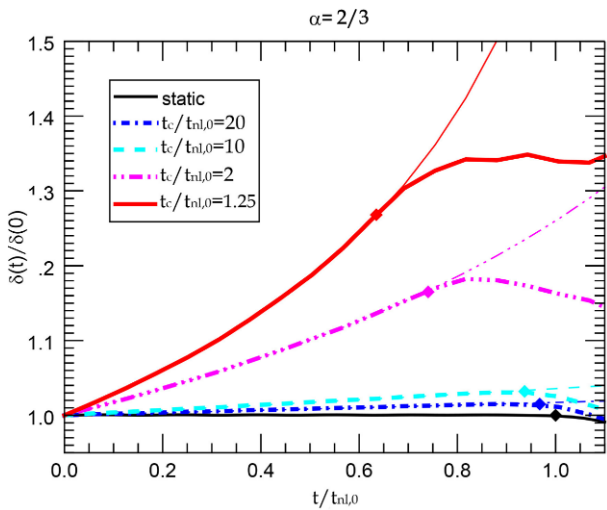
Figure 3. Time evolution of the rms amplitude of density perturbations in a isothermal gas contracting isotropically with the scalefactor of equation (46) with \alpha = 2/3 (case of dynamical contraction) for various values of t_c (thick lines). The time is in units of t_{nl,0} , the non-linear time for the static model. A diamond marks the position of t_{nl} given by equation (47), and thin lines show the evolution of the amplitude in the WKB approximation. For t > t_{nl} shocks are formed and the waves dissipate.
