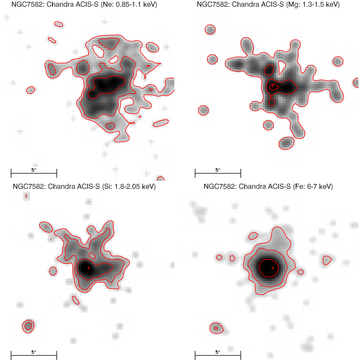
Fig. 6. ACIS-S zeroth order images of NGC 7582 mapping, from top to bottom , the Ne IX-X ( upper left panel ), the Mg XI-XII ( upper right panel ), the Si XIII-XIV ( lower left panel ), and the Fe K \alpha ( lower right panel ) energy ranges. In all the images the red crosses indicate the coordinates of the nucleus (from NED) and the spatial scale is reported at the bottom (note that for NGC 7582 1'' corresponds to 109 pc). The emission appears to be spatially extended in almost all the energy ranges with a different morphology depending on the energy. The emission is progressively less extended with increasing energy and at the Fe K \alpha emission line it is almost consistent with a point-like source, albeit with a weak elongation in the north direction. The Chandra PSF HEW is 0.5''.
