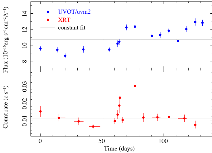
Fig. 4. UVOT/ uvvm2 and XRT light curves of the NGC 4303-O1, identified as a Seyfert 1 galaxy (catalogued as 2XMMJ122137.8+043025). The time zero is set to MET = 412217321 s (2014-01-24). The fit performed on the data with a constant function returns a mean UV flux ( upper panel , aperture with radius = 5 arcsec) of 1.1 \times 10^{-15} erg s^{-1} cm^{-2} \text{\AA}^{-1} , \chi^2 = 242.8 (15 d.o.f.), and a null probability. The fit with a constant function on the X-ray data ( lower panel ) returns a mean rate of 1.06 \times 10^{-2} counts s^{-1} , \chi^2 = 39.15 (14 d.o.f.), and p = 0.0003 .
