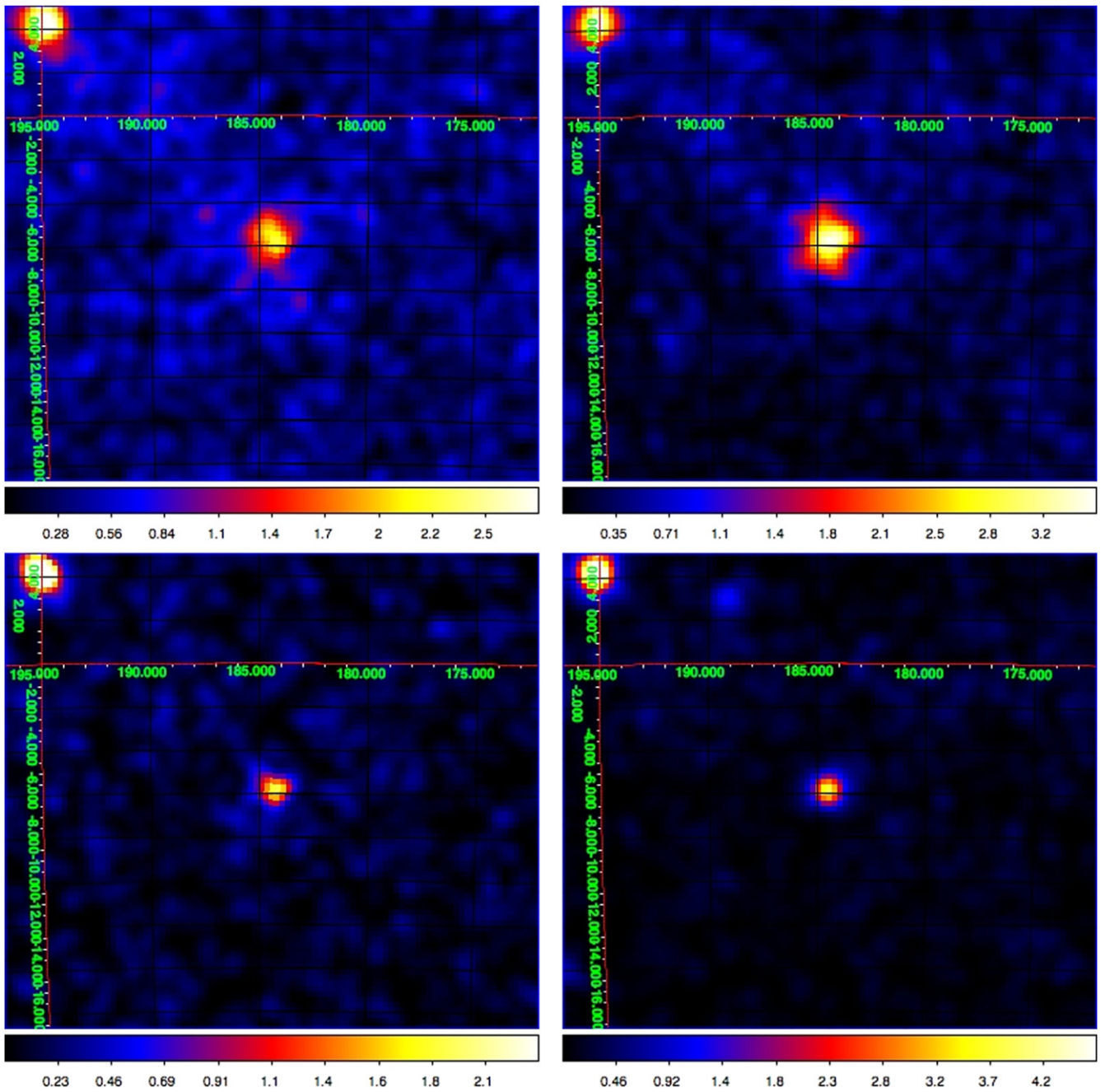
Figure 7. AGILE /GRID (left panels) and Fermi /LAT (right panels) in-flight count maps for the Crab region in the 100–400 MeV and 400–1000 MeV energy bands, respectively. The pixel size is 0\text{.}25 . Note that the color intensity scale is set so that each map has the maximum value of the scale corresponding to the Crab peak counts.
