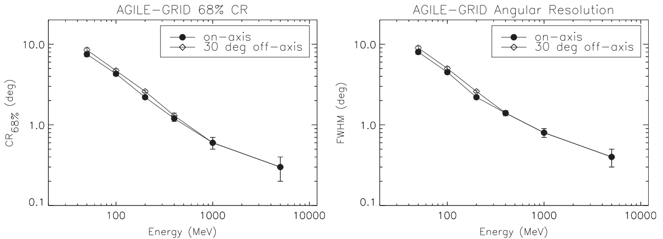
Figure 1. Left panel: AGILE /GRID 68% containment radius vs. photon energy for simulated monochromatic photons of different incident angles. Right panel: angular resolution (FWHM) vs. photon energy, shown for comparison to the CR68.
