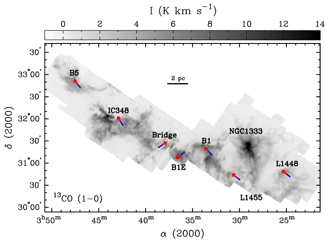
Figure 7. Velocity gradient orientations across Perseus as determined from ^{12}\text{CO} (1–0) observations from COMPLETE (Ridge et al. 2006). Background image shows the integrated intensity map for ^{13}\text{CO} (1–0) using the COMPLETE data. Arrows show the direction of centroid velocities from bluer values to redder values (they are not scaled to the gradient magnitude). We excluded NGC 1333 from this analysis (see text).
