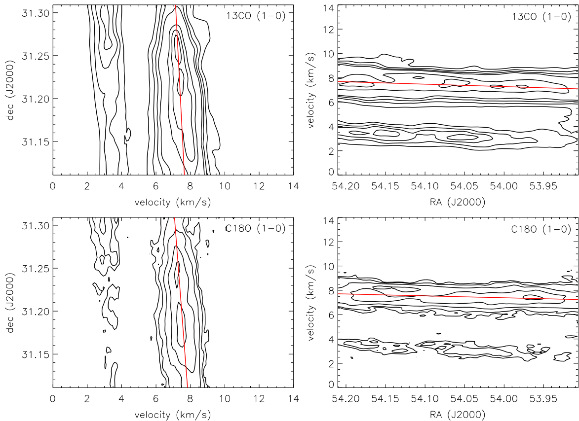
Figure 5. Position–velocity diagram for (top) IRAM ^{13}CO (1–0) and (bottom) IRAM C^{18}O (1–0). Lines were averaged across strips in declination (left) or right ascension (right). For ^{13}CO (1–0), contour levels correspond to average T_{MB} values of 0.5, 1.0, 1.5, 2.0, 4.0, 5.0, and 5.7 K. For C^{18}O (1–0), contours correspond to average T_{MB} values of 0.04, 0.08, 0.2, 0.5, and 1.0 K. The red lines correspond to the weighted mean velocity for T_{MB} > 1.0 K ( ^{13}CO ) or T_{MB} > 0.1 K ( C^{18}O ).
