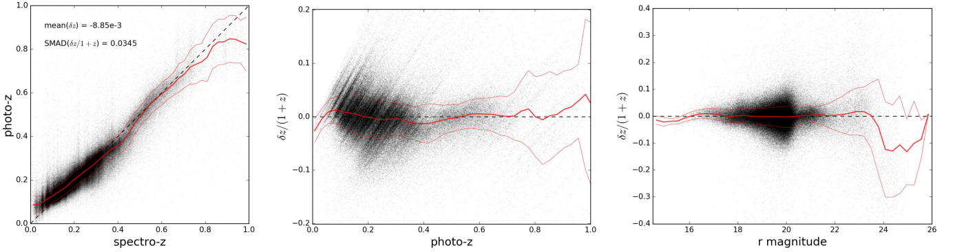
Fig. 5. Performance of the KiDS DR3 ANNz2 photo- z s from the released catalogue as compared to the overlapping spectroscopic samples. Left-hand panel: direct spec- z -photo- z comparison; central panel: photo- z error as a function of photo- z ; right-hand panel: photo- z error as a function of the r -band magnitude. The thick solid line shows the running median while the thin lines encompass the scatter (SMAD). Note different scalings of the \delta z/(1+z) axes. Based on these comparisons, we judge the published photo- z s to be reliable within z_{\text{phot}} < 0.9 and r < 23.5 .
