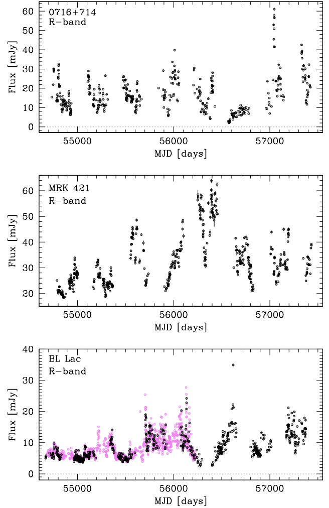
Fig. 2. Nightly averaged R -band light curves (Aug. 2008–Jan. 2016) for 0716+714 and MRK 421 from Tuorla Observatory, and for BL Lac obtained combining nightly averaged data from Tuorla (black) and the WEBT observations (violet). The light curves are not host galaxy subtracted. The reported light curves match with the Fermi monitoring. Error bars are, in most cases, smaller than symbol size.
