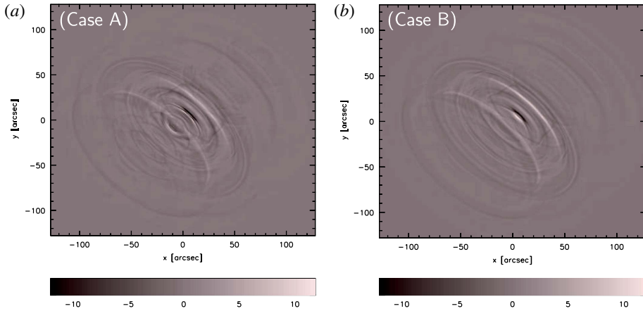
FIGURE 2. Appearance of wisps at radio frequency in case A (a) and case B (b). Wisps maps are obtained by subtracting images of the emission separated by a time interval of approximately 2 months. Outward motion of the wisps can be observed as consecutive darker and lighter arcs.
