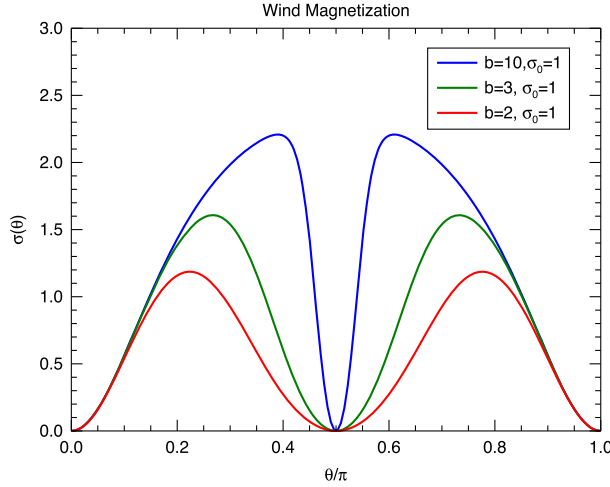
FIGURE 4. Shape of the wind magnetization \sigma(\theta) for the value of \sigma_0 = 1 employed in our 3-D simulation and for three values of b . The upper (blue) curve is the case with a narrow striped wind region used here, with \sigma_{eff} = 1.5 , while the bottom (red) curve refers to a case that approximately reproduces the magnetization function as in the B3D run of Porth et al. (2014b).
