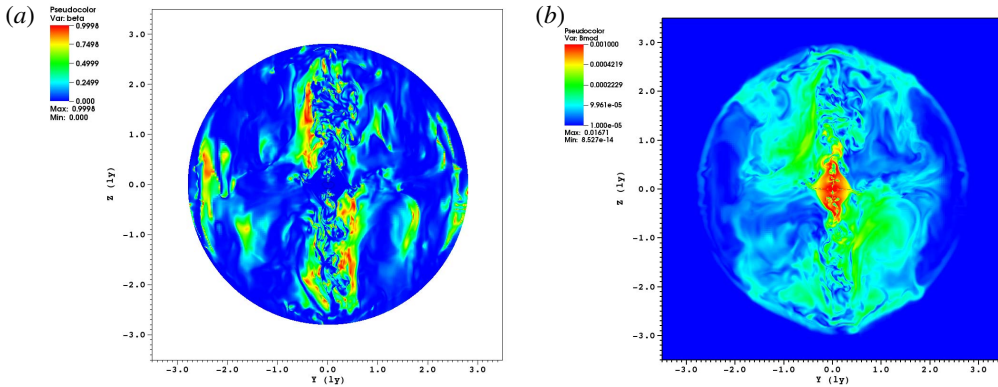
FIGURE 8. (a) The ratio of the polar to the total magnetic field magnitude in a 2-D slice of the data cube at t=250 yr. Data are also cropped within a circle of radius equal to the nebular radius (2.8 ly) for ease of interpretation. As expected, the polar component is mostly important near the polar jets. (b) Image of the 2-D distribution of the total magnetic field magnitude in the 0, y, z plane, shown in units of Gauss at the time 250 yr. The magnetic field appears to be stronger close to the TS, where the mean value is around 1 mG.
