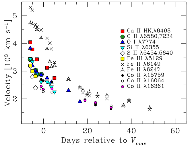
Figure 12. Velocity evolution of the absorption minima of a selection of spectral lines with minimal line blending in the spectra of SN 2014ck. The typical formal error of the velocities is \sim 200 km s ^{-1} . The blending of lines can produce a systematic shift of features and increase the uncertainty at least to \sim 1000 km s ^{-1} .
