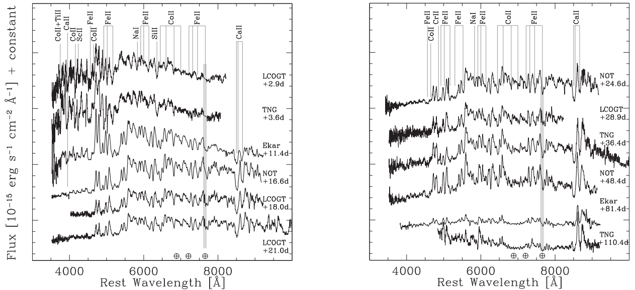
Figure 9. Spectral evolution and line identifications. Phases are reported relative to V-band maximum. Left-hand panel: spectra between +2.9 d and +21 d. Right-hand panel: spectra between +24.6 d and +110.4 d. Wavelength is in the rest frame and the positions of major telluric absorption features are marked with the \oplus symbol (in particular the vertical grey band marks the strong O 2 A-band absorption at 7600 Å).
