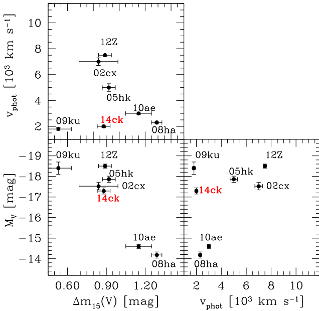
Figure 16. Scatter plots of \Delta m_{15}(V) , M_V and photospheric velocities v_{ph} derived around +10 d for several well studied SNe Ia (see Narayan et al. 2011, their fig. 3).
