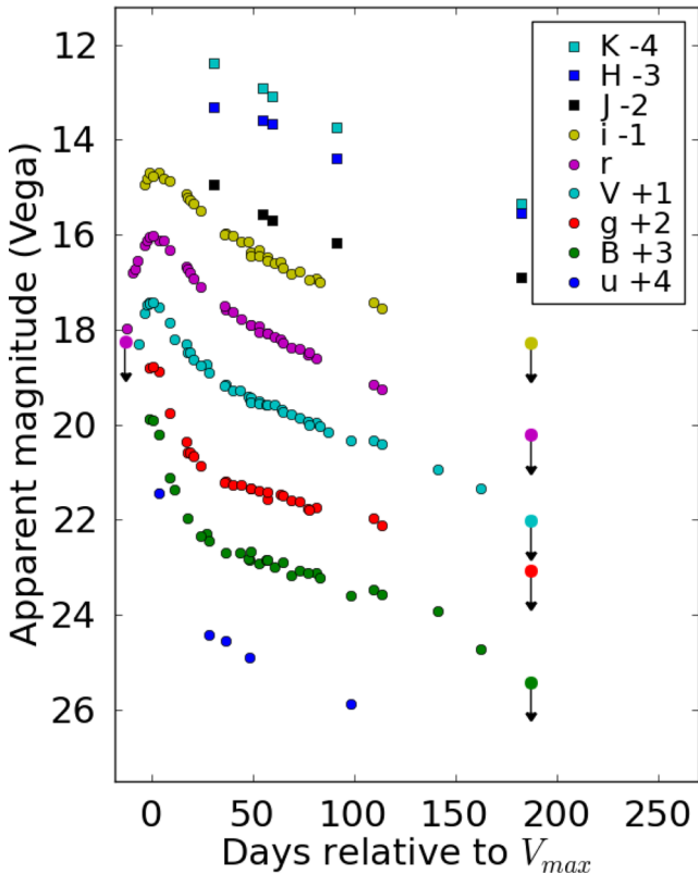
Figure 3. Light curves of SN 2014ck in the uBVgriJHK bands. Sloan ugri AB magnitudes have been here plotted as Vega magnitudes for uniformity with BVJHK bands, following Blanton & Roweis (2007). For clarity, the light curves have been shifted vertically as indicated in the legend. The uncertainties for most data points are smaller than the plotted symbols. The last BVgri photometric epoch is an upper limit.
