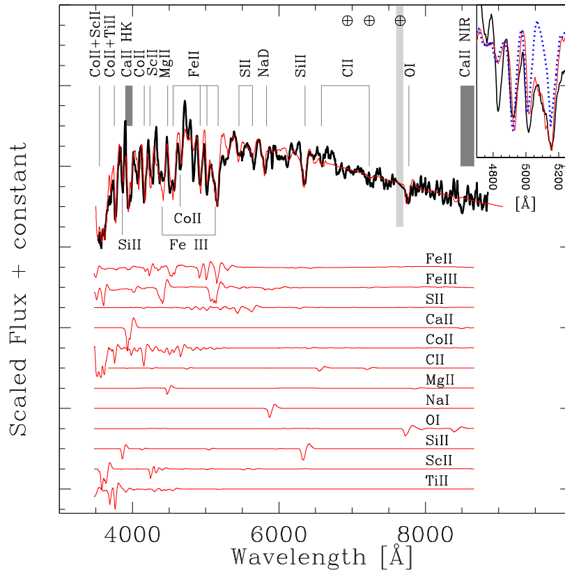
Figure 10. Optical spectrum of SN 2014ck at +1.7 d (black) and our best-fitting synov synthetic spectrum (red). The contribution of each ion is also shown. Major telluric features are indicated with the \oplus symbol (in particular the vertical grey band marks the strong O 2 A-band absorption at 7600 Å). The insets on the right of the plot show the regions around Fe III \lambda 4404 (bottom) and Fe III \lambda 5129 (top) with a synthetic spectrum calculated without Fe III overplotted (dotted blue).
