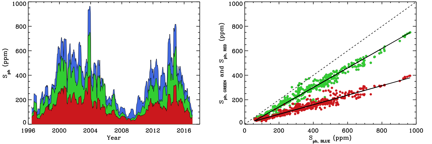
Fig. 6. Left panel: photospheric activity proxies, S_{\text{ph}} (in ppm), for each of the BLUE, GREEN, and RED channels of the VIRGO/SPM observations as a function of time. Right panel: photospheric activity proxy, S_{\text{ph}} from the VIRGO/SPM GREEN (GREEN dots) and RED (red dots) channels as a function of the photospheric index, S_{\text{ph}} , from the BLUE channel. The solid lines correspond to weighted linear regressions between the data, and the dashed line represents the 1:1 correlation.
