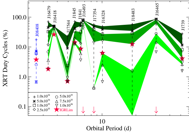
Figure 7: The XRT duty cycle (2–10 keV) as a function of orbital period and for a range of 2–10 keV luminosities (see legend, in units of \text{erg s}^{-1} ) in black. Only points above 0.1% are shown. Since the period of J08408 is currently unknown (see Table 1 Col. 2 for the values adopted for the rest of the sample), we arbitrarily place it at an orbital period of about two days and mark it in blue. The shaded areas mark the loci of the XRT duty cycle defined by contiguous luminosities. The red filled stars represent the XRT duty cycle at the INTEGRAL sensitivity for each object (the downward-pointing arrows are consistent with 0). The data on IGR J16493–4348 and AX J1845.0–0433 are presented here for the first time, the rest are adapted from Romano et al. (2014a).
