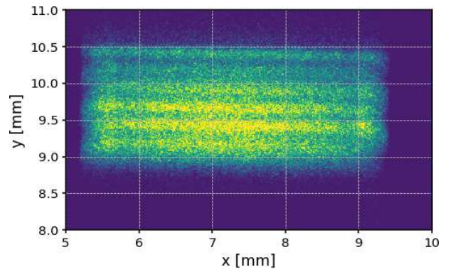
Figure 23: Example of the scan with the T-collimator. The image is acquired with the ICE test imager. This is equivalent to the middle panel of Figure 20. Strips are the tracks of the spot during the scan.
