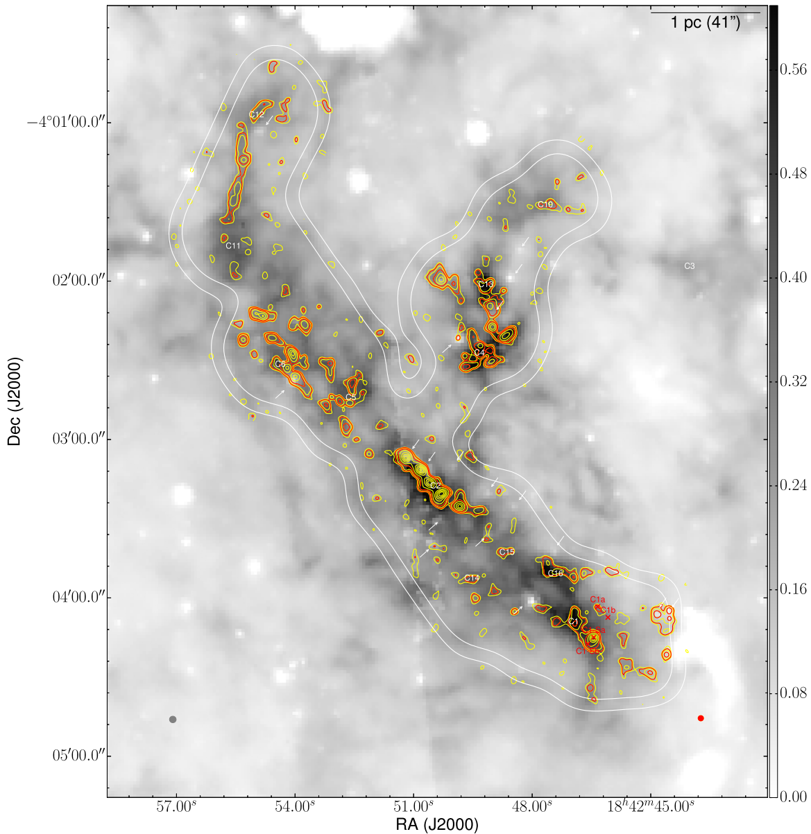
Figure 1. Grayscale: MIREX mass surface density map from BTK14 (scale in \text{g cm}^{-2} ). The angular resolution of the map is shown as the gray filled circle at the lower left. “C1, C2, C3...” label extinction peaks from BTK14. The white arrows point to possible embedded protostars that show as local enhancements in the 8 \mu\text{m} image, which produce local “holes” in the MIREX map. Contours: ALMA 1.3 mm continuum mosaic. The contours range from S/N = 2, 3, 5, 10, 20, 40, 60, \dots with the rms noise at map center \sigma_{\text{center}} \sim 0.2 \text{ mJy beam}^{-1} . The two red contours highlight S/N = 3 and 10. The synthesized beam is shown as the red filled ellipse at the lower right. The two white enclosing contours show primary-beam responses of 0.3 (outer) and 0.5 (inner). (The data used to create this figure are available.)
