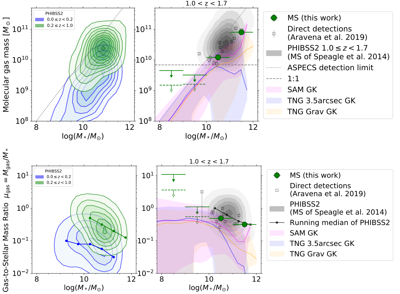
Figure 11. The same diagrams as Figure 5, to show our results in the context of previous studies of the molecular gas content. Note that the MS galaxies here are classified based on the prescription of Speagle et al. (2014) following Tacconi et al. (2018). Thus, the data points and the MS boundaries are slightly shifted compared to Figure 5 in the main text. The distributions of PHIBSS2 galaxies at lower redshifts are displayed in the left panels (color-coded by redshift as given in the legend). Most of the PHIBSS2 galaxies at z \sim 0 are from xCOLD GASS (Saintonge et al. 2017).
