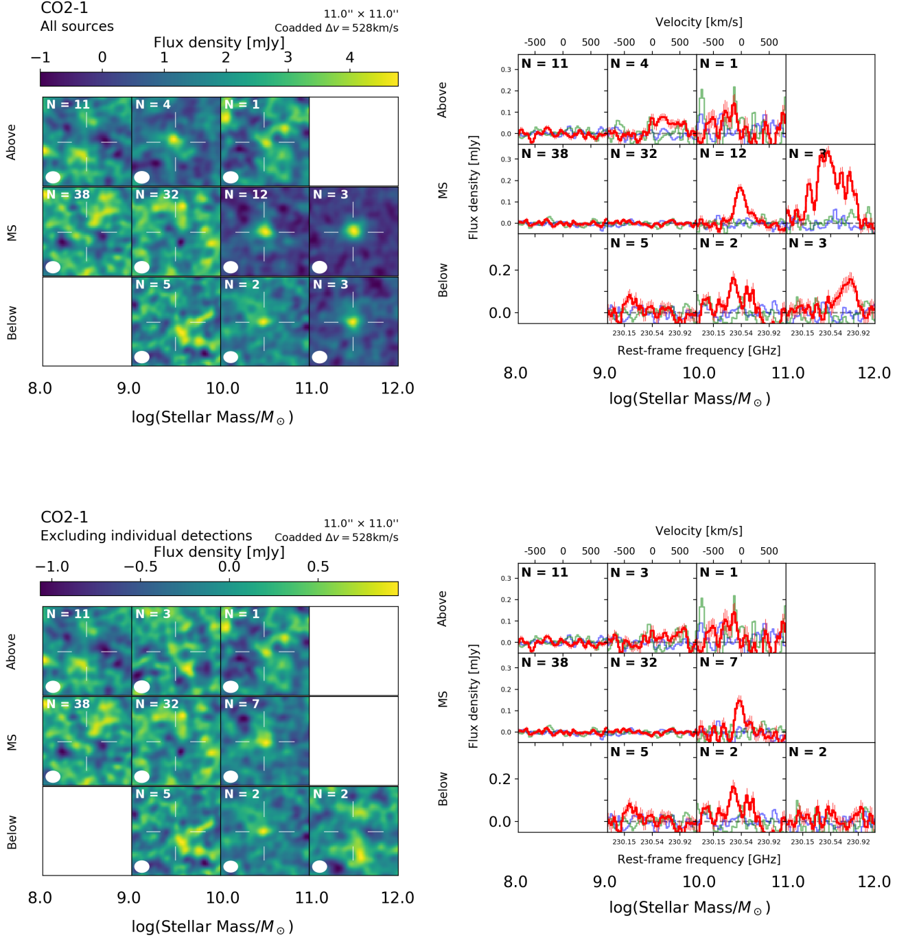
Figure 4. Resulting stacked 2D images (left) and 1D spectra (right) in the bins of SSFRs (above, on, and below the galaxy main-sequence, as discussed in §3.2; y-axis) and stellar masses (x-axis). The upper and lower two panels show the results of including and excluding the individually reported direct CO(2-1) detections, respectively (Aravena et al. 2019; Boogaard et al. 2019). The 2D images are coadded between 230.335 \leq \nu_{\text{rest}}/\text{GHz} \leq 230.741 ( \Delta v = 528 \text{ km s}^{-1} ) and the white ellipses indicate the mean of the beam size. The 1D spectrum is extracted from the central spaxel (the red solid line). Spectra extracted with random redshifts in place of the MUSE position and with random positions at the correct MUSE redshift are shown by the light blue and green lines, respectively (§3.1).
