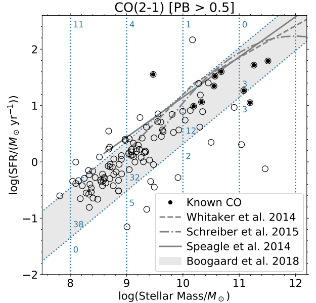
Figure 3. SFR- M_* relation of our CO(2-1) stacking sample. The gray filled band shows the main-sequence relation and its intrinsic scatter for MUSE-detected galaxies (at z = 1.43 , Boogaard et al. 2018). The gray solid, dashed and dashed dotted lines are the main-sequence relations from Speagle et al. (2014) (which is used for PHIBSS2 Tacconi et al. 2018, see also Appendix D), Whitaker et al. (2014) and Schreiber et al. (2015), respectively. The blue vertical and diagonal dotted lines show the divisions of the bins that we used for stacking. The numbers at the top left of each grid are the counts of galaxies in the bin. The filled circles indicate the galaxies which have CO(2-1) line detections in the ASPECS blind search (see §3.2).
