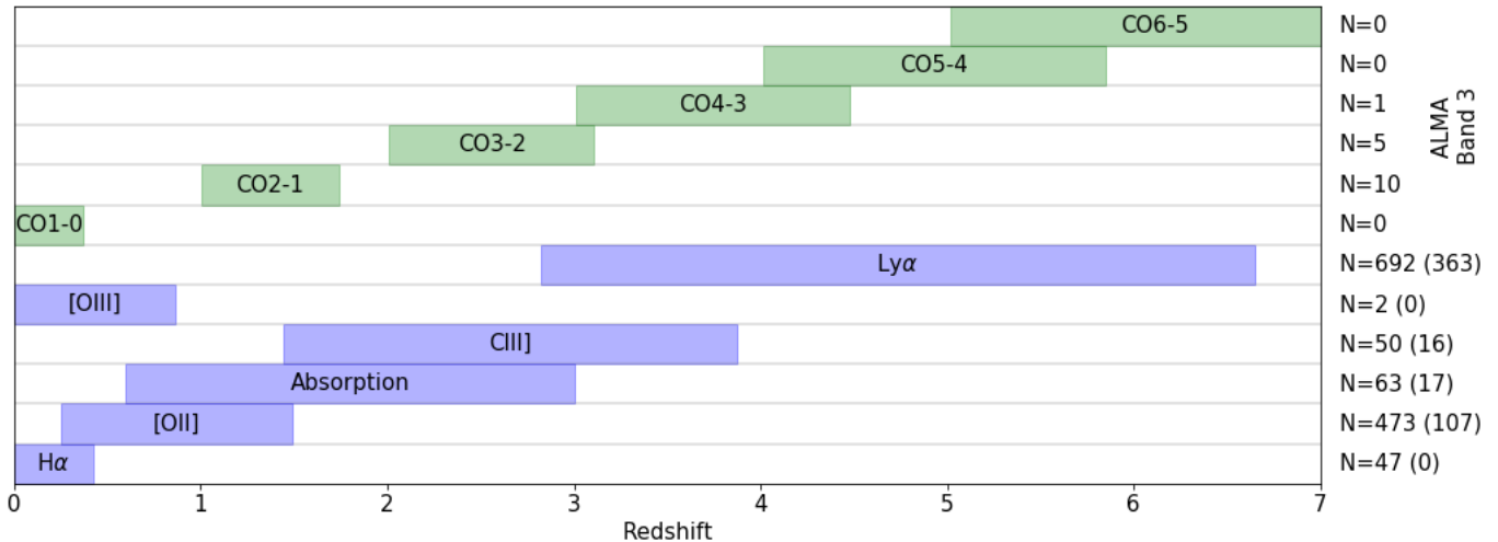
Figure 1. The redshift coverages of the MUSE (blue) and ASPECS (green) HUDF surveys. The numbers of ASPECS directly detected sources and MUSE sources with a secure redshift measurement are listed on the right hand side (There are also nine and two sources classified as “stars” and “others”, respectively, Inami et al. 2017). The numbers in parentheses are the MUSE sources whose locations are in the region of LP primary beam response > 50\% for each CO emission. The absorption features detected with MUSE include C IV, Fe II, Mg II. The analysis presented in this work focuses on the stacking frequencies that correspond to the CO(2-1), CO(3-2), CO(4-3), CO(5-4), and CO(6-5) lines.
