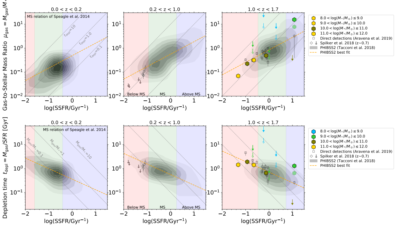
Figure 12. The same diagrams as Figures 6 and 7 in the main text, but lower redshift bins are also shown, following Figure 11. Again, the main-sequence relation of Speagle et al. (2014) is used here instead. Thus, the data points and the MS boundaries are slightly shifted compared to Figures 6 and 7. The light pink, green, and blue background colors indicate the regions of below, on, and above the main-sequence relation at \log(M_*/M_\odot) = 10 , respectively. The orange dashed lines are the best-fit lines for the PHIBSS2 sample (Tacconi et al. 2018).
