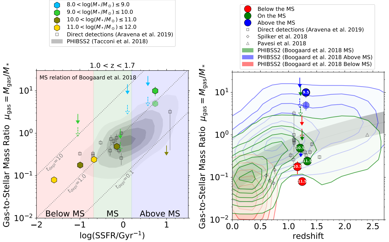
Figure 6. [Left] Gas-to-stellar mass ratios as a function of SSFR. The symbols are the same as in Figure 5, but now we show the entire sample, below, on, and above the main-sequence relation, color-coded with their stellar masses as indicated in the legend. The same as the other figures involving molecular gas mass estimates, we use \alpha_{\text{CO}} = 3.6 M_\odot (\text{K km s}^{-1} \text{pc}^2)^{-1} for galaxies in the \log(M_*/M_\odot) > 10 bins and 7.2 and 10.8 for the \log(M_*/M_\odot) \sim 9.5 and 8.5 bins, respectively (see §5.1). We also show the estimates based on a constant \alpha_{\text{CO}} = 3.6 M_\odot (\text{K km s}^{-1} \text{pc}^2)^{-1} in the lower mass bins with the dashed symbols for reference. The data points are centered on the mean values of the parameters on the x-axis. The three diagonal gray dotted lines represent constant depletion time scales of 0.1, 1.0, and 10 Gyr from the bottom to the top. The background pink, green, and blue filled colors indicate the below, on, and above the main-sequence relation of Boogaard et al. (2018) for a galaxy at \log(M_*/M_\odot) = 10.0 . A version using the main-sequence relation of Speagle et al. (2014) is shown in Appendix D. [Right] The evolution of gas-to-stellar mass ratios. The symbols are the same as Figure 5 but now we include galaxies above and below the main-sequence relation: above (blue), below (red), and on the MS relation (green). The values inside each symbol indicate the corresponding stellar mass bins in log scale. The PHIBSS2 galaxies classified as above, below, and on the MS by the main-sequence relation of Boogaard et al. (2018) are also depicted as red, green, and blue contours, respectively. The gray curve in the background and its shaded region show the evolutionary track of main-sequence galaxies from Tacconi et al. (2018).
