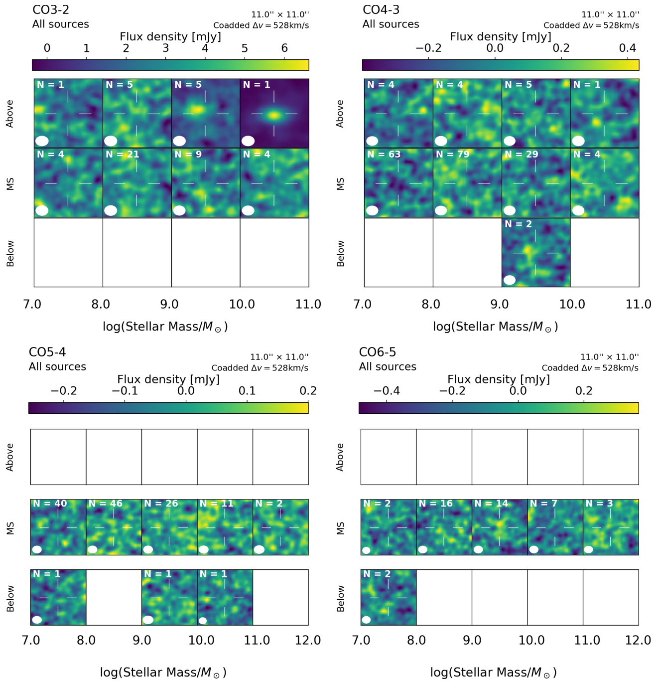
Figure 9. The stacked results of CO(3-2), CO(4-3), CO(5-4), and CO(6-5), shown in the same manner as the left panel in Figure 4, at top left, top right, bottom left, and bottom right, respectively. No significant detections in the stacks are reported.
