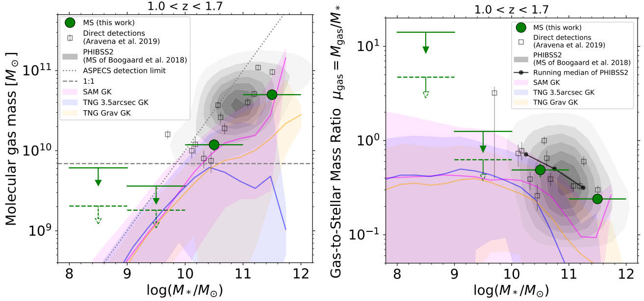
Figure 5. [Left] Molecular gas mass as a function of stellar mass of the main-sequence galaxies in this study. We use \alpha_{\text{CO}} = 3.6 M_{\odot} (\text{K km s}^{-1} \text{pc}^2)^{-1} for galaxies in the \log(M_*/M_{\odot}) > 10 bins and 7.2 and 10.8 for the \log(M_*/M_{\odot}) \sim 9.5 and 8.5 bins, respectively, to obtain molecular gas mass (see §5.1). We also show the estimates based on a constant \alpha_{\text{CO}} = 3.6 M_{\odot} (\text{K km s}^{-1} \text{pc}^2)^{-1} in the lower mass bins with the dashed symbols for reference. The large green circles are from the stacked CO detections and the downward-pointing arrows are the 3\sigma upper limits. The squares indicate the ASPECS CO detections from the blind search (Aravena et al. 2019). The PHIBSS2 galaxies (Tacconi et al. 2013, 2018; Freundlich et al. 2019), classified as MS galaxies with the MS relation of Boogaard et al. (2018) over 1.00 \leq z \leq 1.74 , are shown as the gray contours for comparison to our results. We also display the model predictions of molecular gas mass from SC SAM (pink line and shading, which indicate the median and 2\sigma scatter, respectively), IllustrisTNG with the 3.5arcsec aperture (blue), and IllustrisTNG with the Grav aperture (beige) from Popping et al. (2019). [Right] Molecular gas-to-stellar mass ratio is presented instead as a function of stellar mass. The symbols are the same as in the left panel. The black line with dots shows the running median of the gas-to-stellar mass ratios of the PHIBSS2 sources lying on the MS of Boogaard et al. (2018) (gray contours; see also Tacconi et al. 2018).
