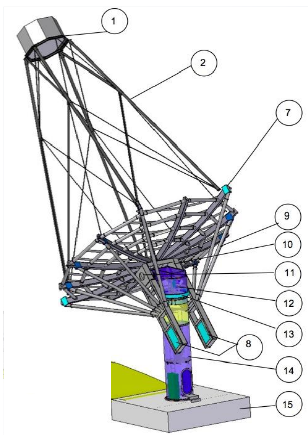
Figure 1: Schematic drawing of the MST.
