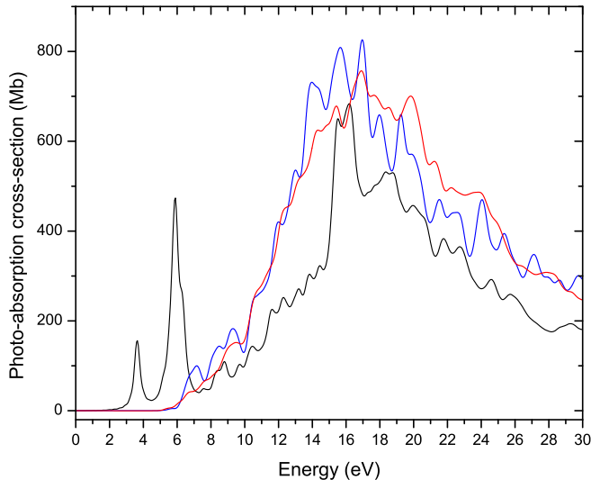
Figure 5. Comparison between the photoabsorption cross-section for neutral coronene ( C_{24}H_{12} , black line, Mallocci et al. (2007)) and for fully superhydrogenated coronene ( C_{24}H_{36} , blue and red lines). All extra H atoms are either attached to one of the face of the molecule (red line) or at alternate faces (blue line).
