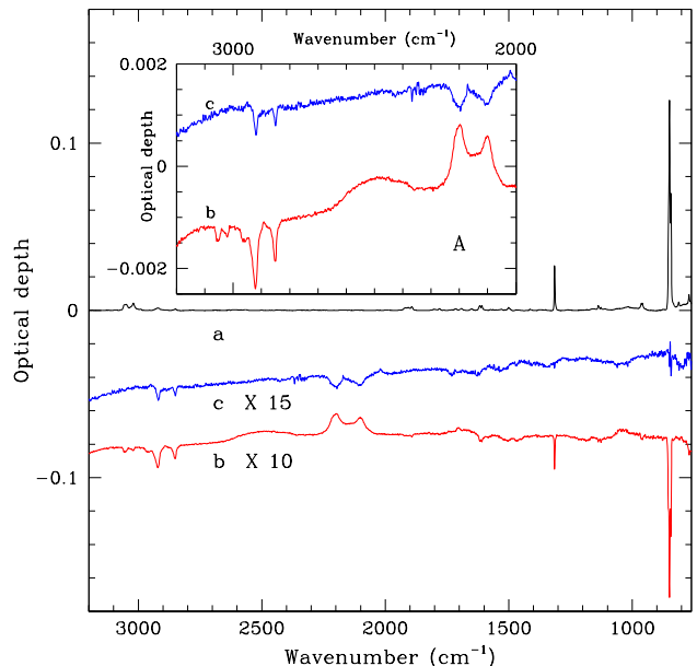
Figure 1. IR spectrum of COR03 film (a), after hydrogenation through exposure to 3.4 \times 10^{18} \text{ D atoms cm}^{-2} (b) and subsequent UV irradiation with 1.2 \times 10^{19} \text{ photons cm}^{-2} (c). The spectrum of the hydrogenated sample is shown after subtraction of the initial spectrum, while the spectrum after UV irradiation is shown after the subtraction of that of hydrogenated coronene. The difference spectra are offset for clarity. Inset A: the traces b and c are zoomed in the region where C-H and C-D stretching bands fall.
