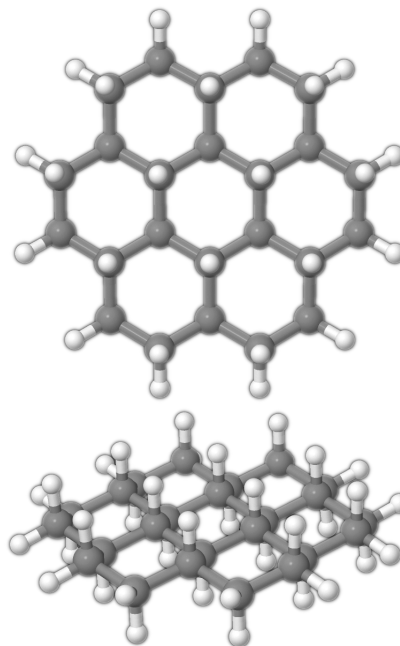
Figure 4. Structure of C_{24}H_{36} with H atoms on alternating sides of the distorted carbon plane of coronene, from two viewing angles
